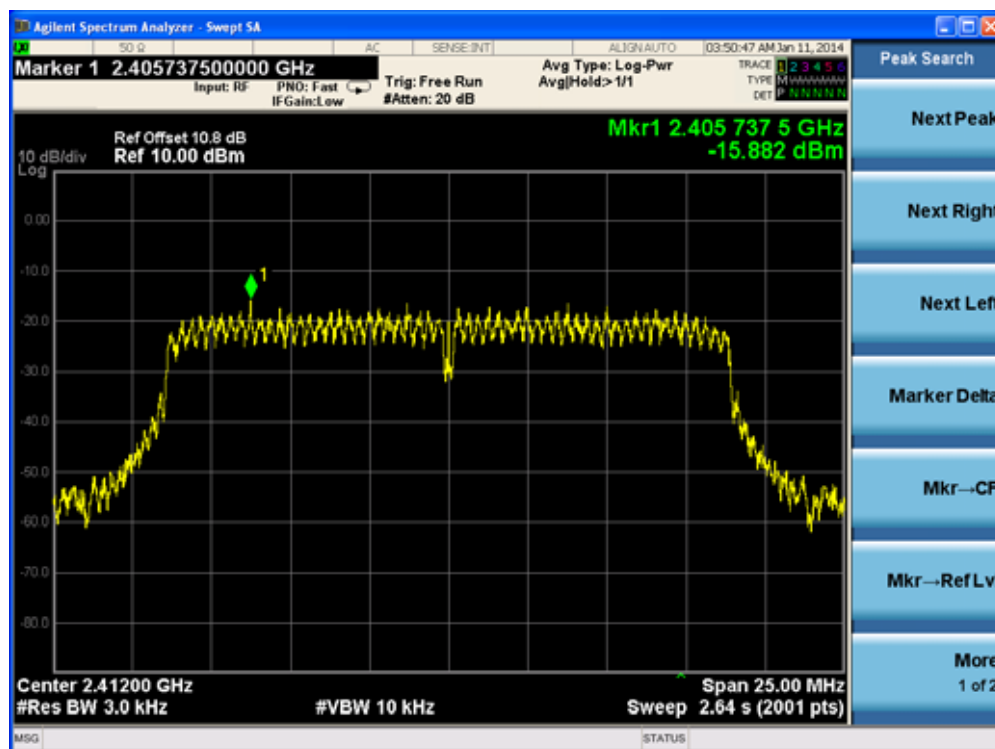
Channel 01 (2412MHz)-Ant 0
