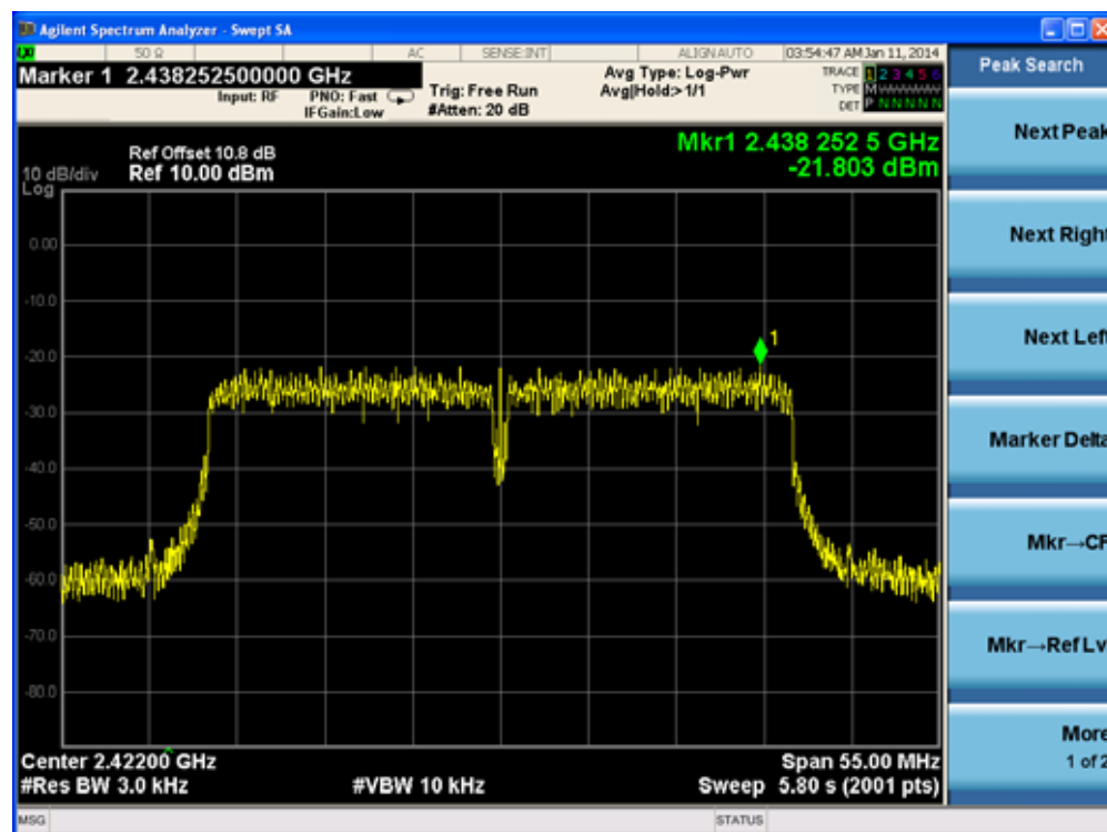
Channel 03 (2422MHz)-Ant 0
