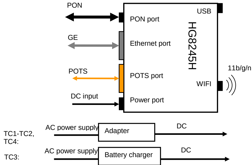
Figure 7.: Test configuration (TC1 ~ TC4)
