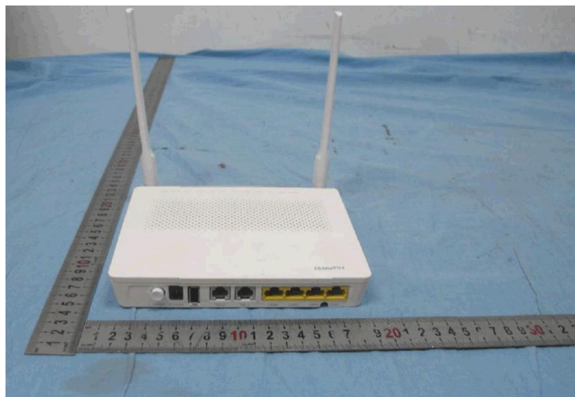
Figure 1. EUT appearance
