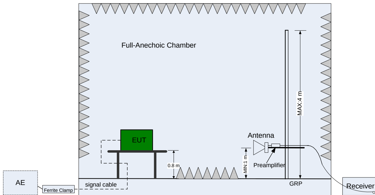
Figure 12. Test set-up of radiated disturbance (above 1 GHz)
