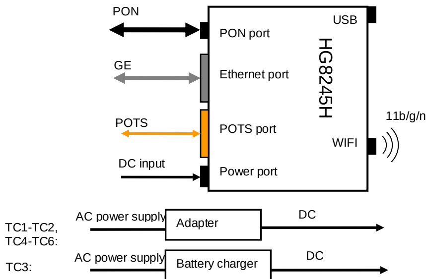
Figure 9.: Test configuration (TC1 ~ TC6)
