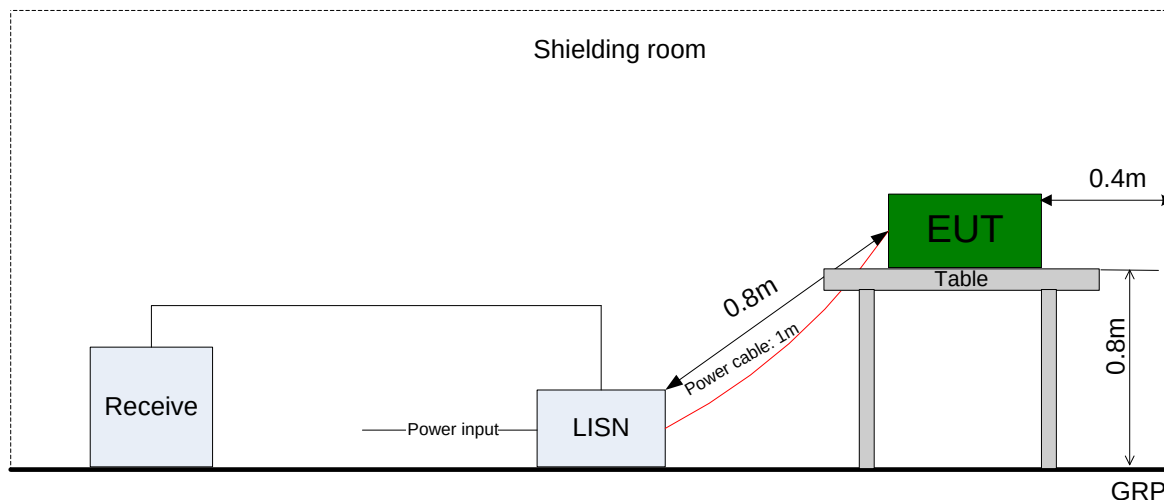
Figure 13. Test set-up of conducted disturbance for AC power port
