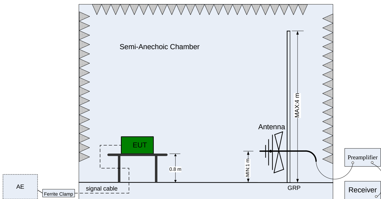
Figure 11. Test set-up of radiated disturbance (30 MHz-1 GHz)
