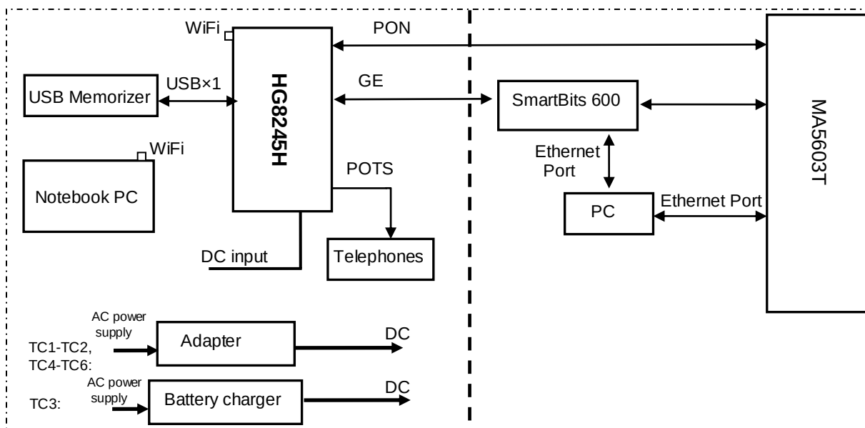
Figure 10. Test connection of TC1 to TC6
