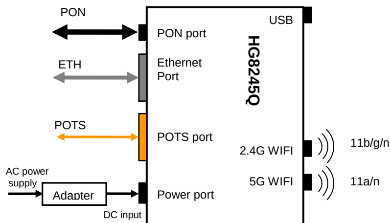
Figure 4. : Test configuration
