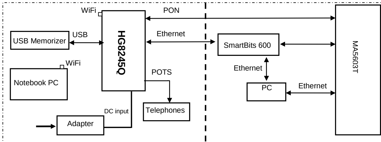
Figure 5. Test connection of TC1-TC2
