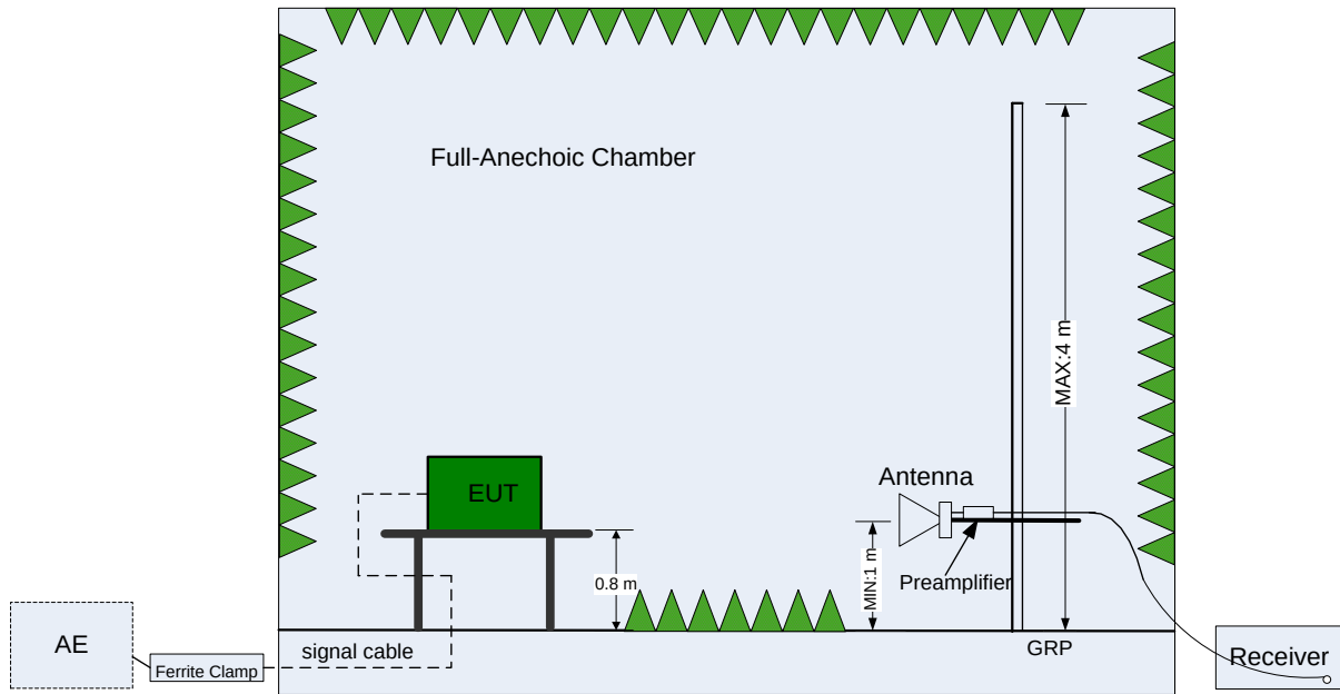
Figure 7. Test set-up of radiated disturbance (above 1 GHz)
