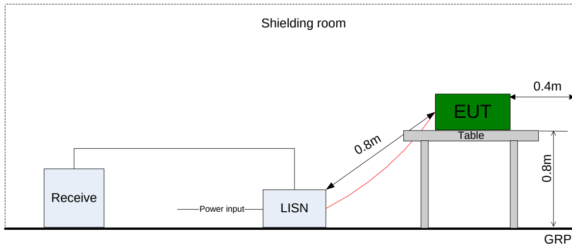
Figure 8. Test set-up of conducted disturbance for AC power port
