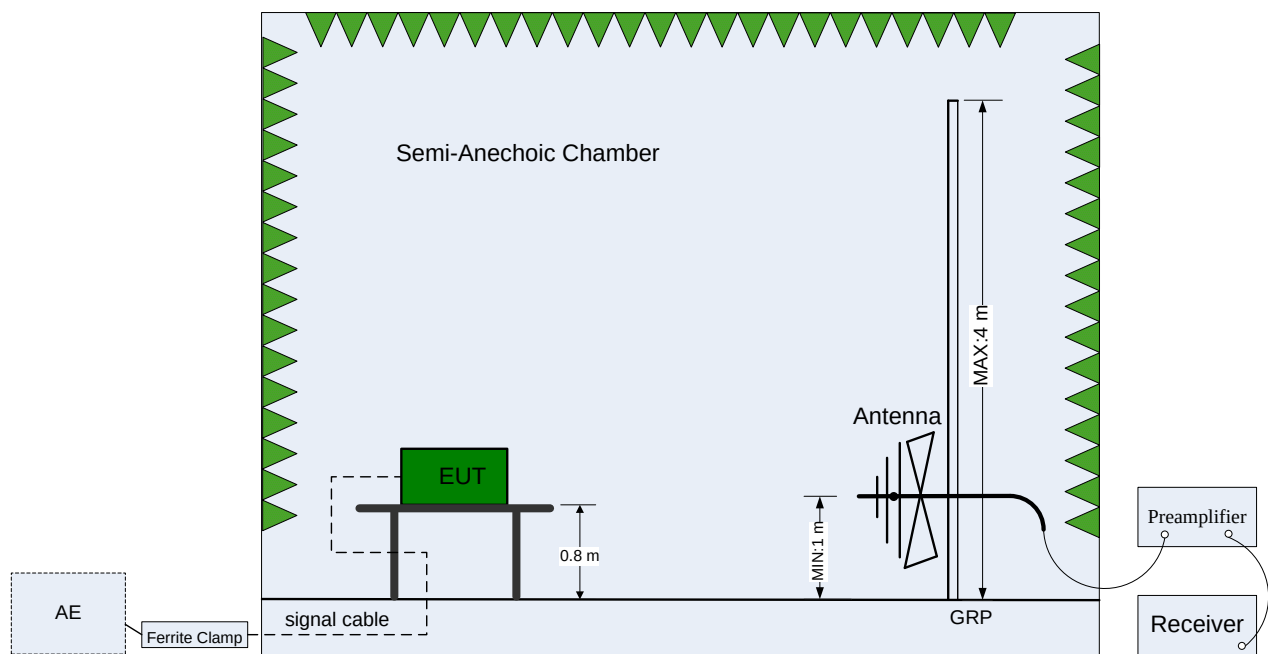
Figure 6. Test set-up of radiated disturbance (30 MHz-1 GHz)
