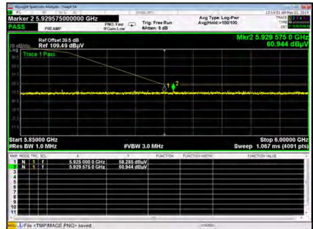
Band III 11ac40 CH142 Peak
