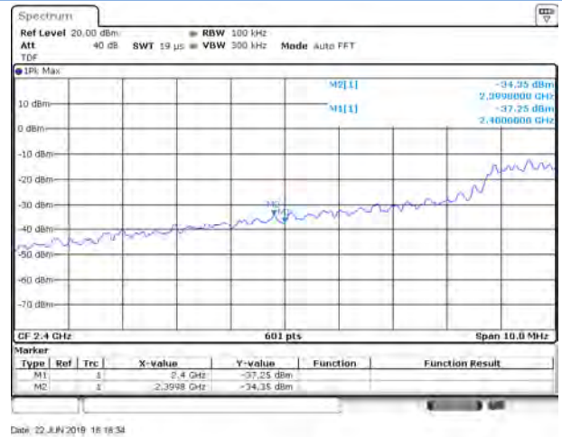
802.11n-40 MHz CHANNEL 3, Reference level
