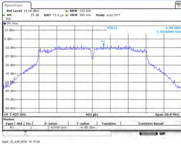
802.11n-40 MHz CHANNEL 3, Carrier level
