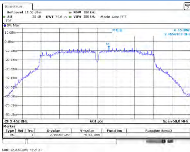
802.11n-40 MHz CHANNEL 9, Carrier level
