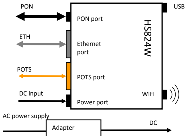
Figure 3. : Test configuration
