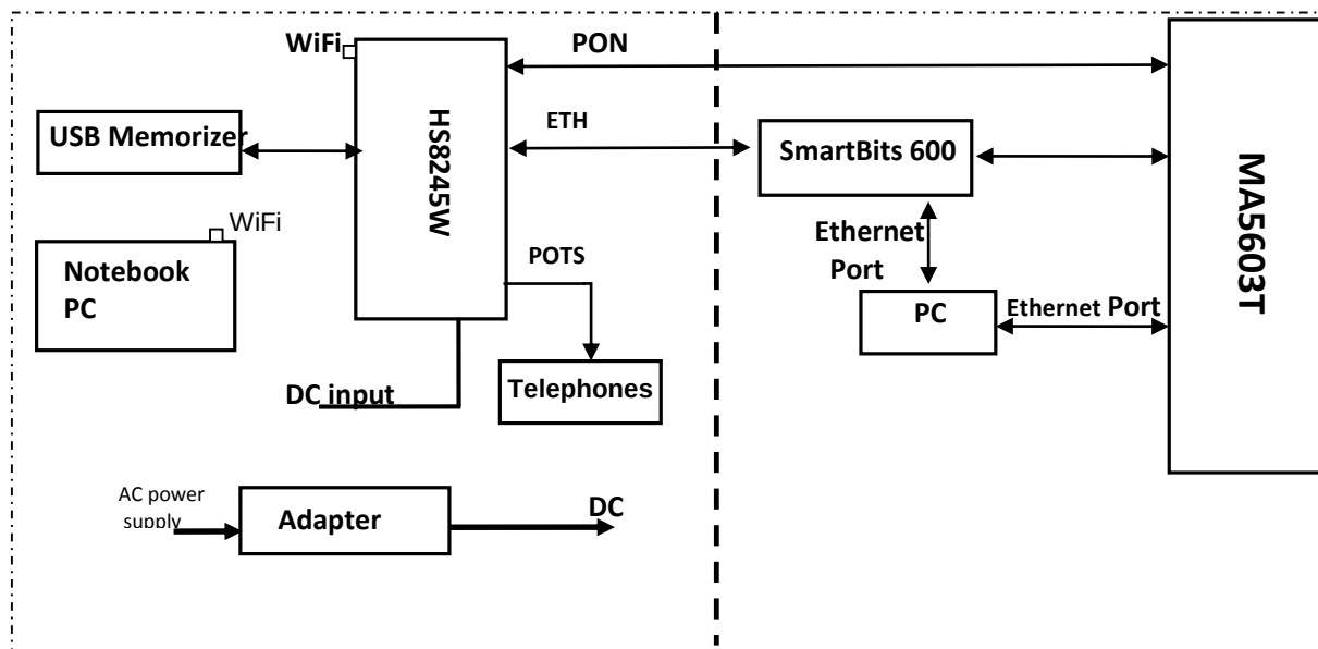
Figure 4. Test connection
