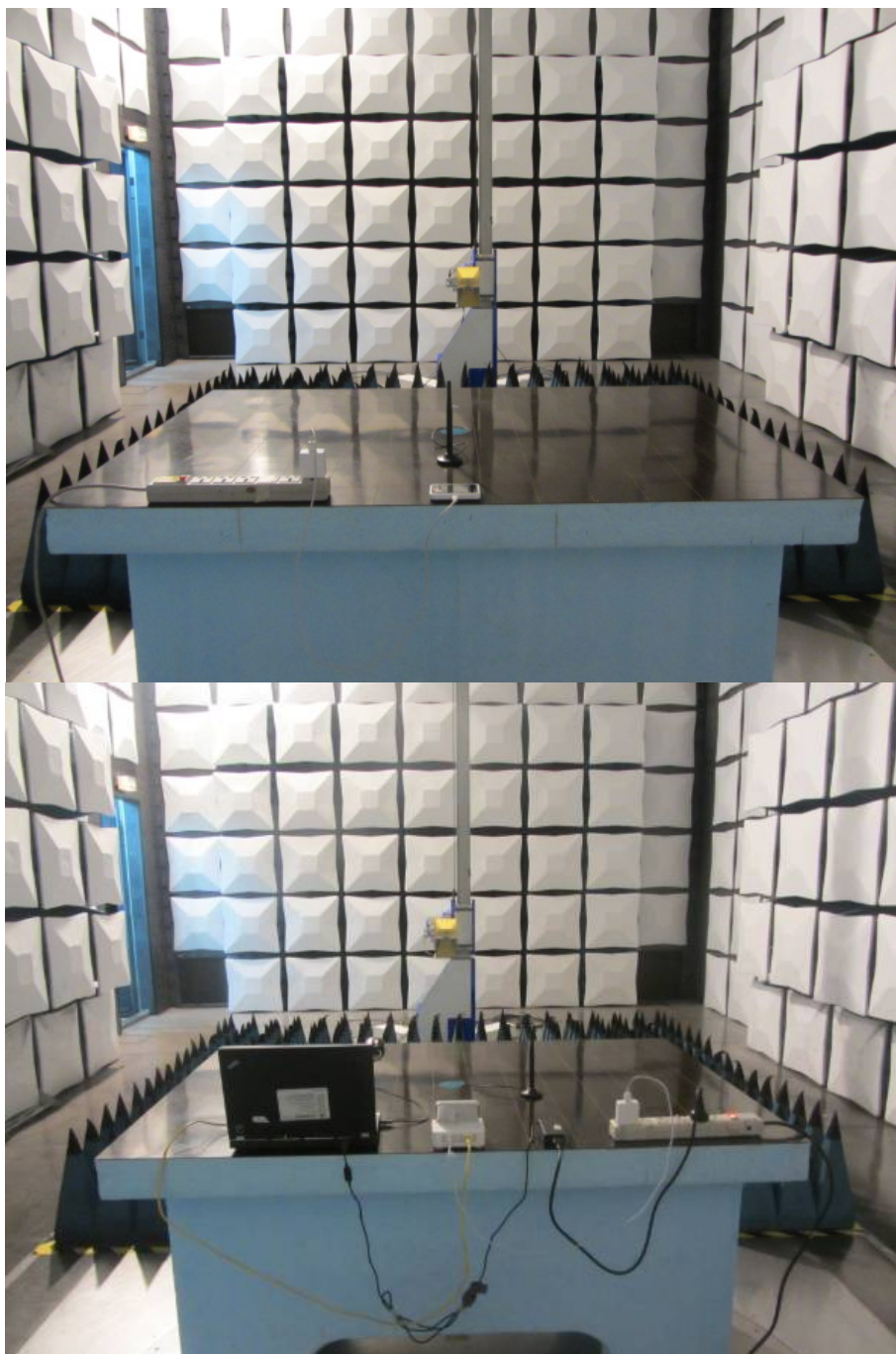
Radiated Disturbance (above 1GHz)
