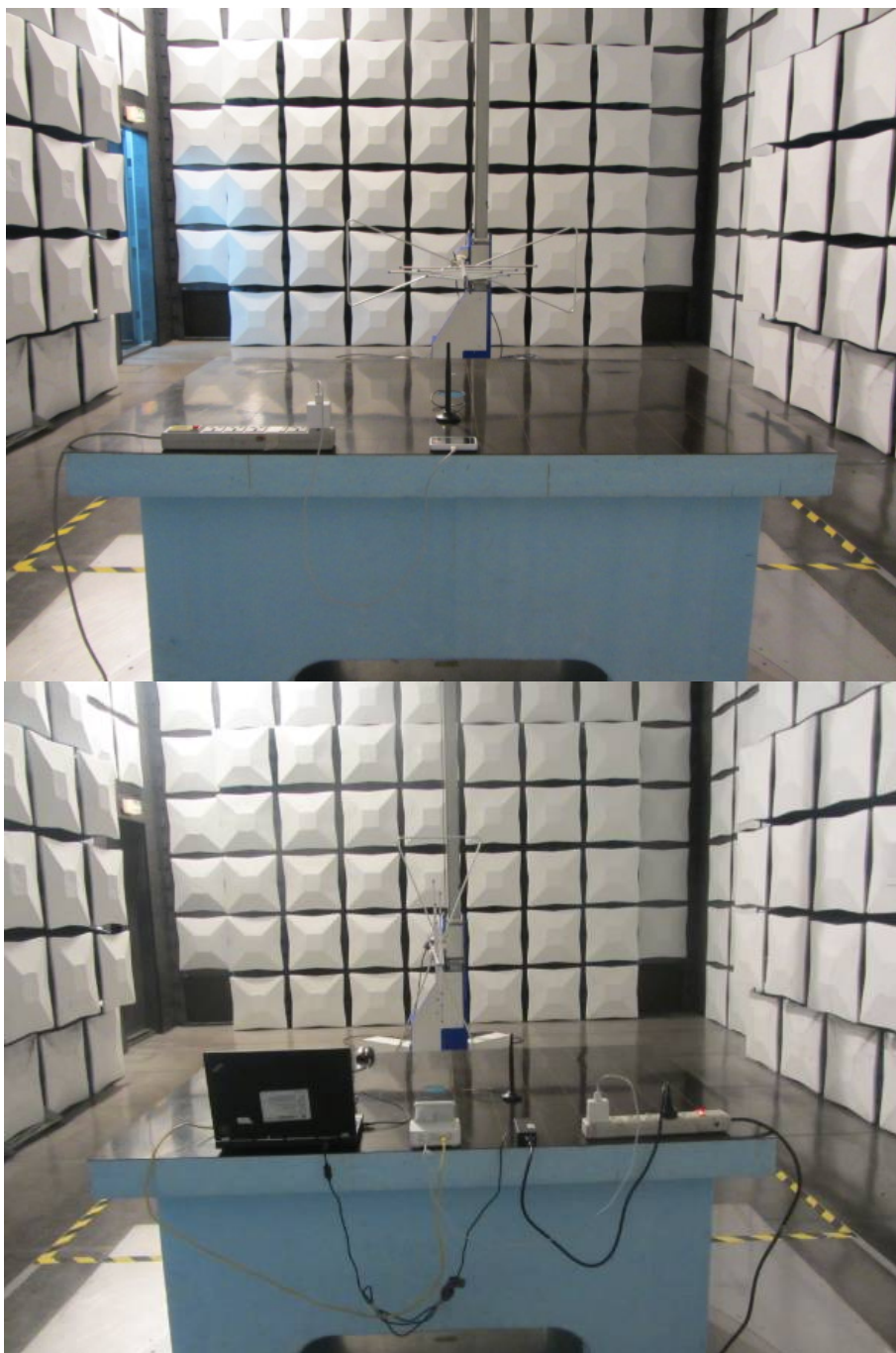
Radiated Disturbance (30MHz-1GHz)
