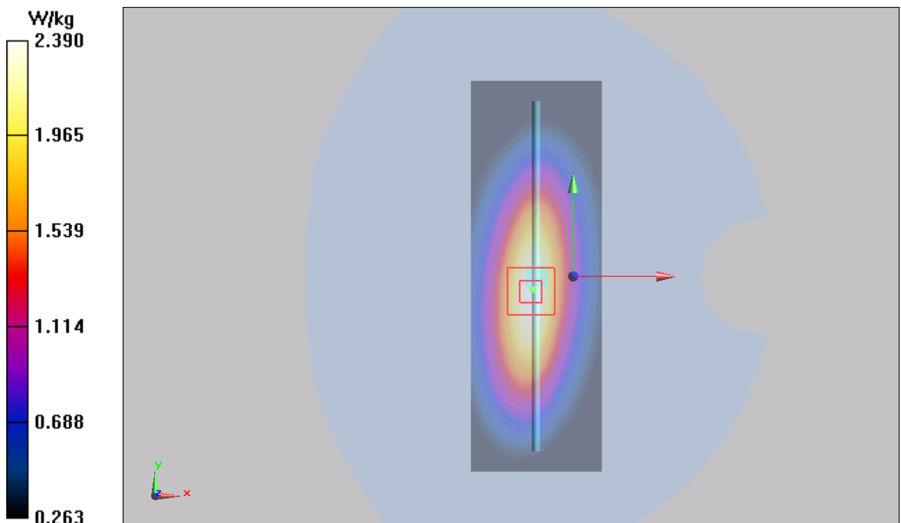
Figure 7 System Performance Check 750MHz 250mW
