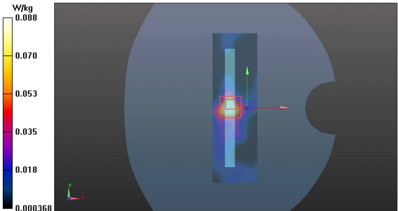
Figure 56 802.11ac Test Position 5 Channel 58
