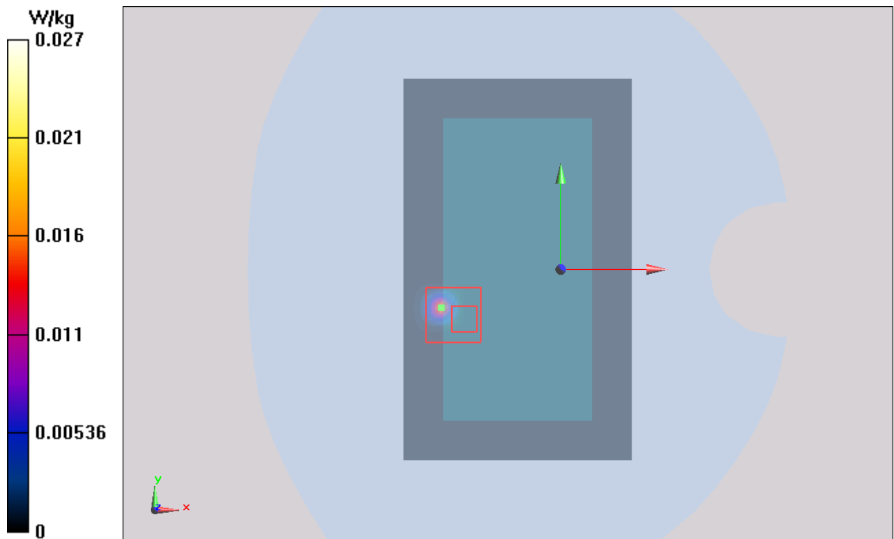
Figure 47 802.11a Test Position 2 Channel 36
