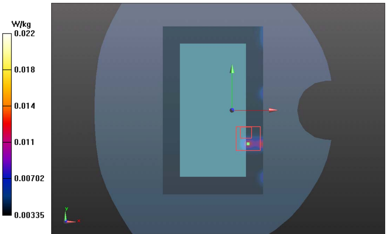
Figure 60 802.11a Test Position 1 Channel 52
