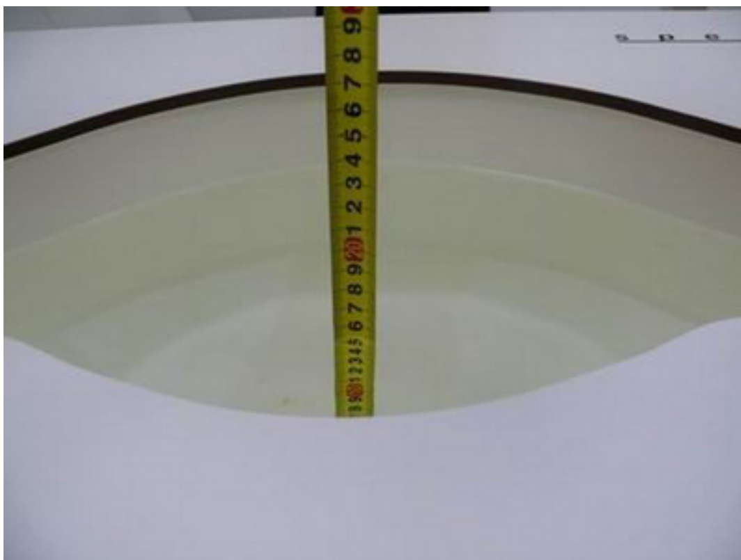
Picture 7: Liquid depth in the flat Phantom (5600 MHz, 15.3cm depth)
