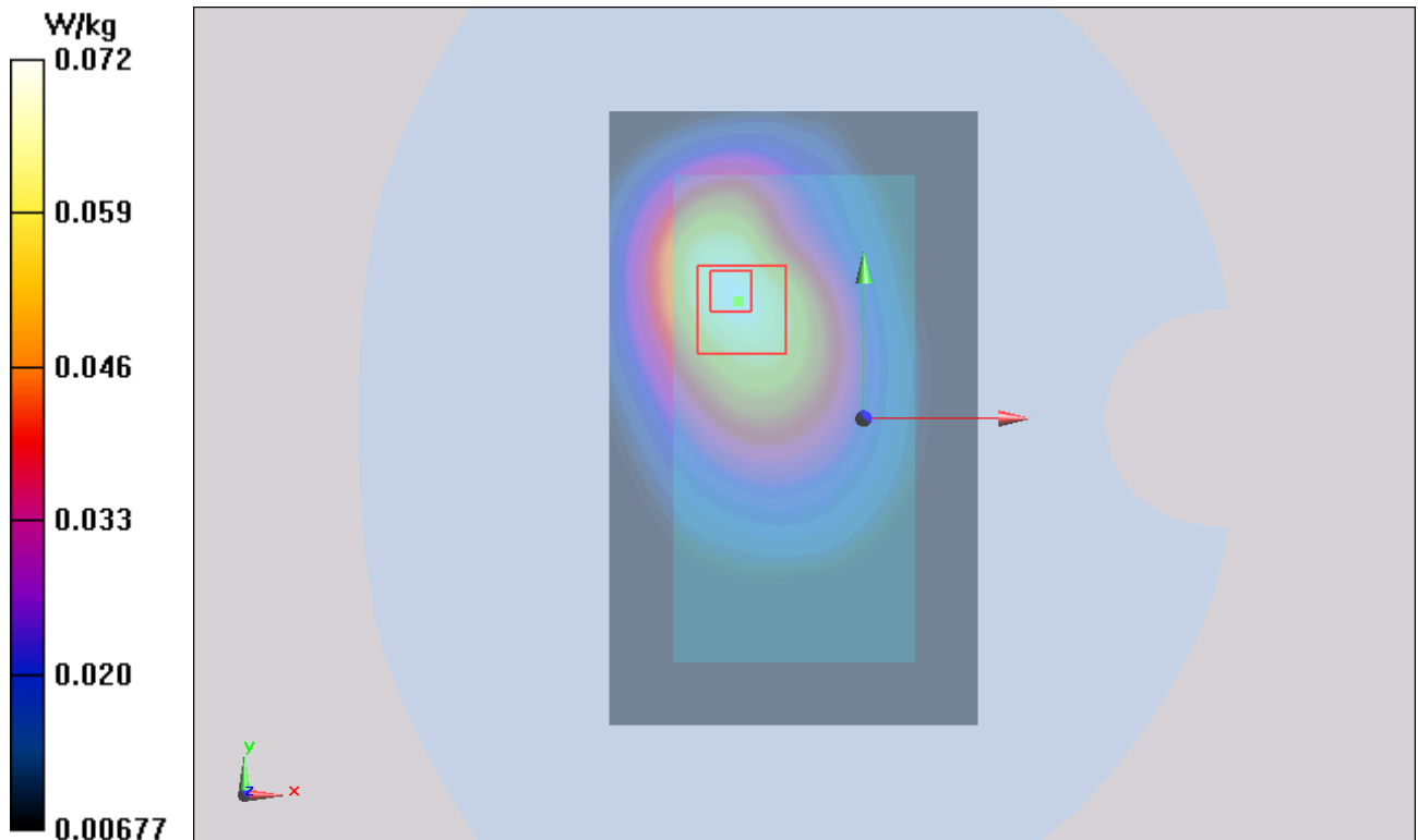
Figure 36 LTE Band 17 with Test Position 2 Channel 23780
