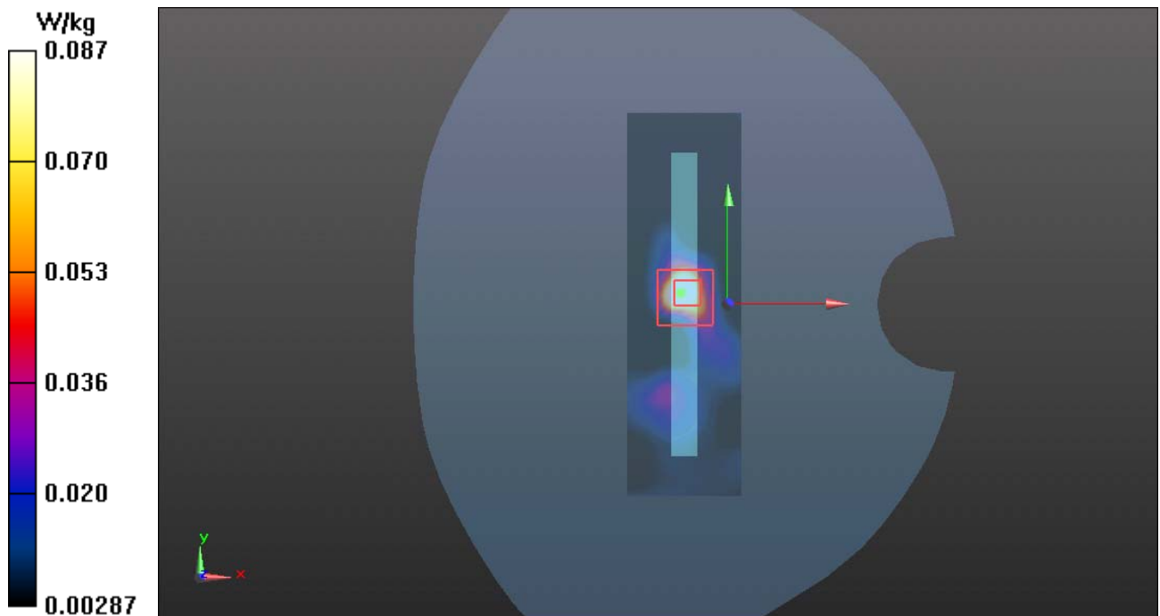
Figure 55 802.11ac Test Position 5 Channel 42
