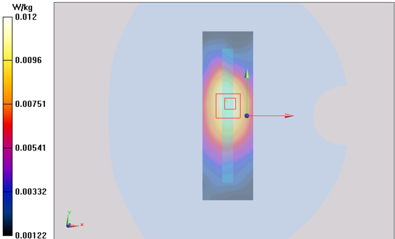
Figure 38 LTE Band 17 with Test Position 5 Channel 23780
