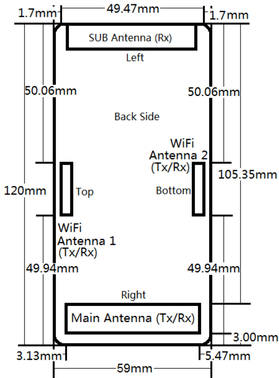
Mobile Hotspot Sides for SAR Testing
