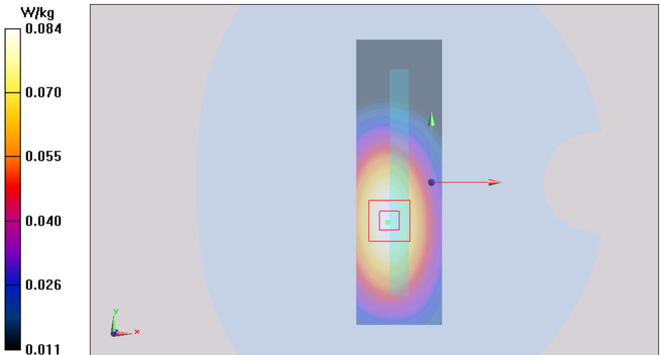
Figure 29 UMTS Band V with Test Position 6 Channel 4183
