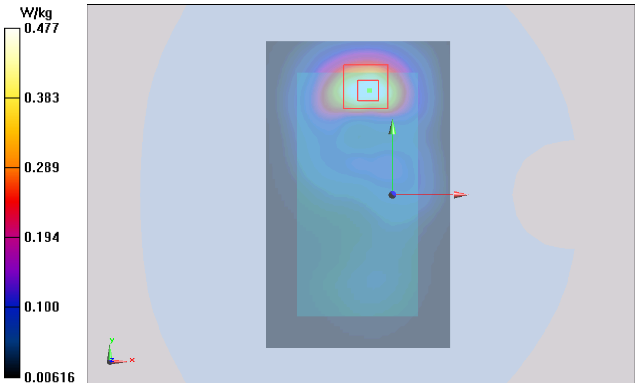
Figure 17 UMTS Band II with Test Position 2 Channel 9400
