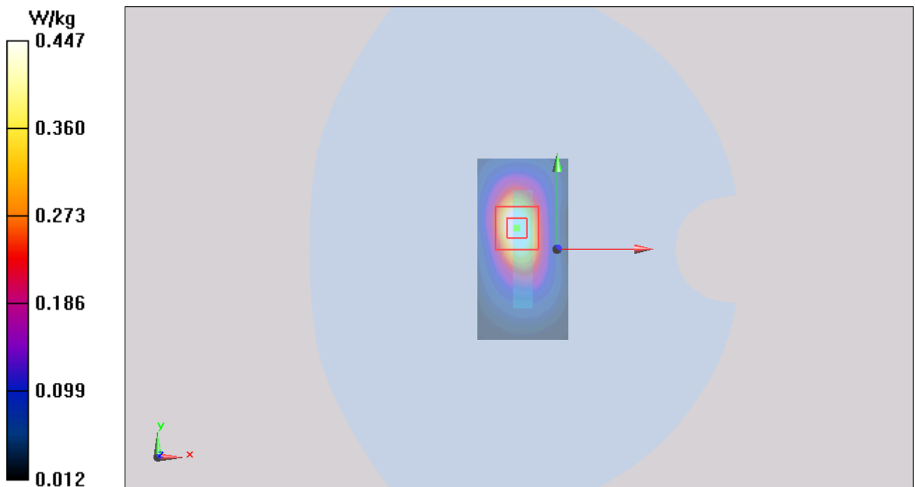
Figure 21 UMTS Band II with Test Position 4 Channel 9262
