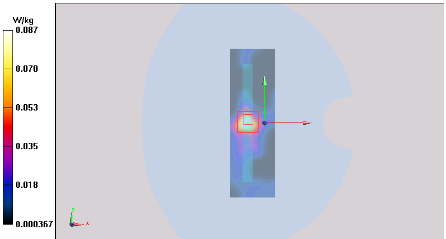
Figure 51 802.11a Test Position 5 Channel 56
