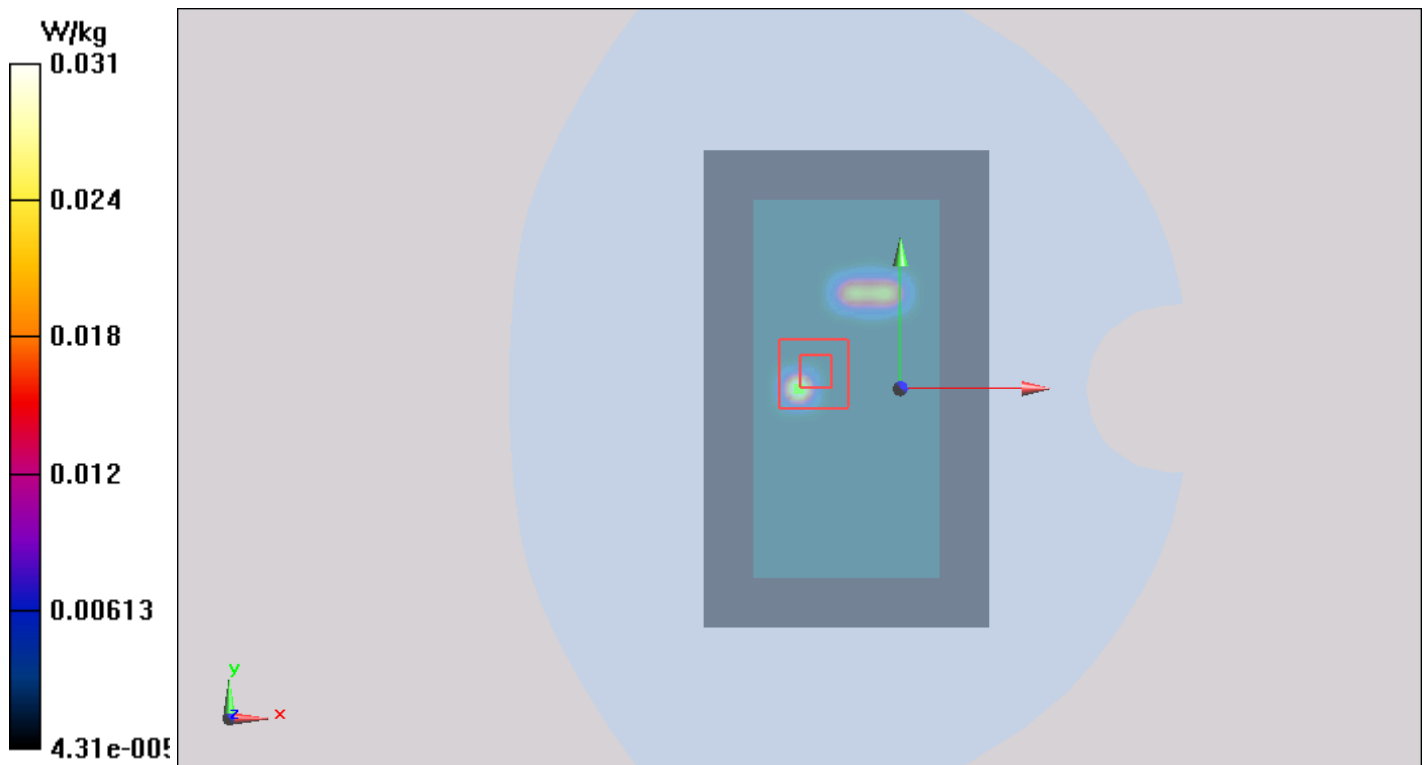
Figure 67 802.11ac Test Position 2 Channel 56
