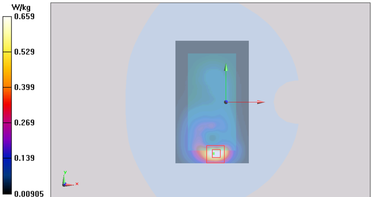
Figure 15 UMTS Band II with Test Position 1 Channel 9262
