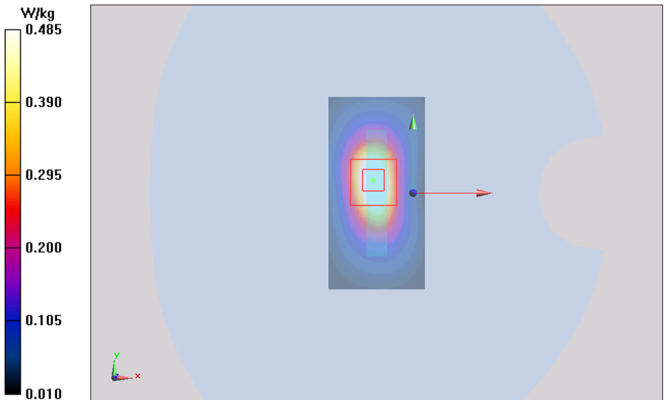
Figure 20 UMTS Band II with Test Position 4 Channel 9400
