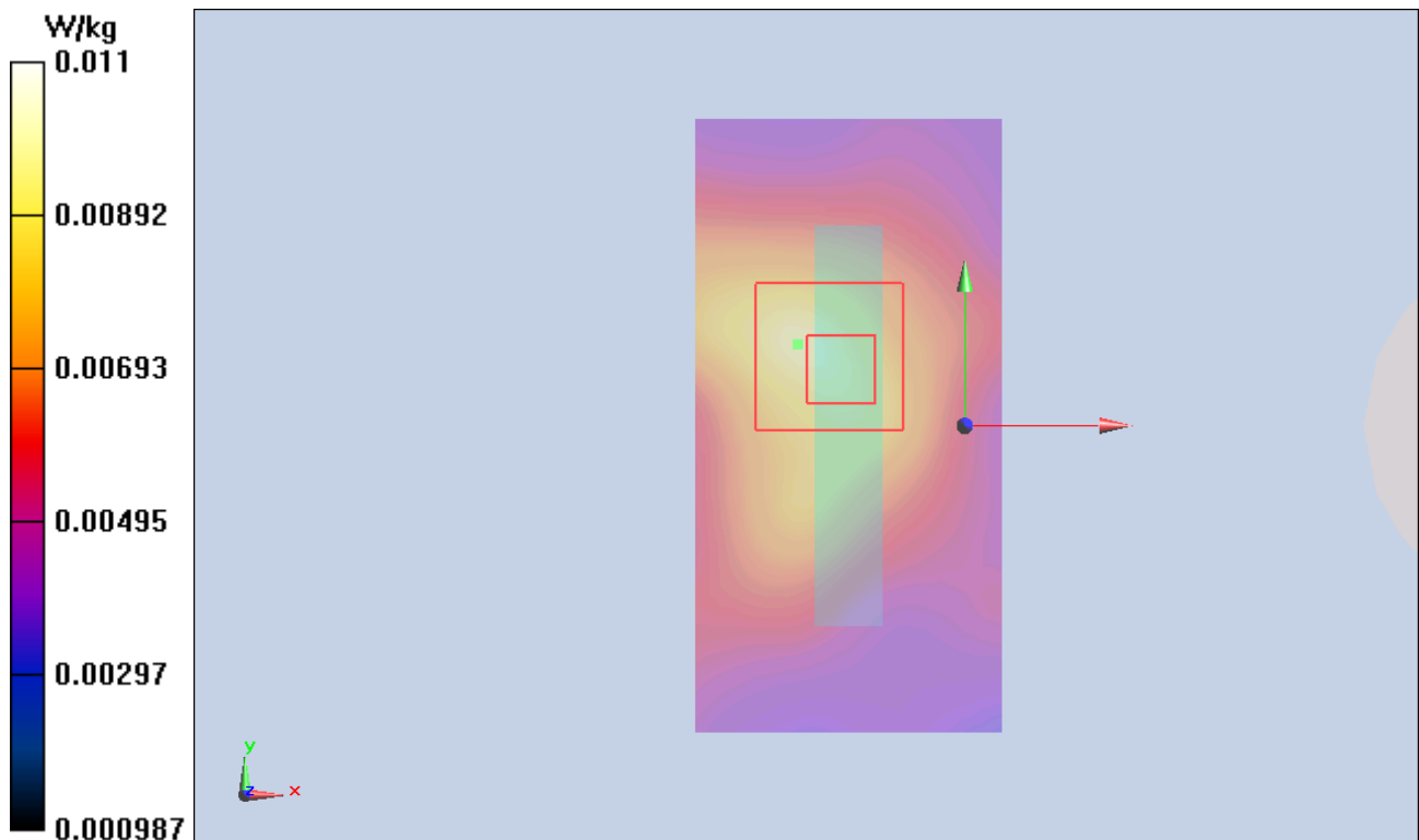
Figure 27 UMTS Band V with Test Position 4 Channel 4183
