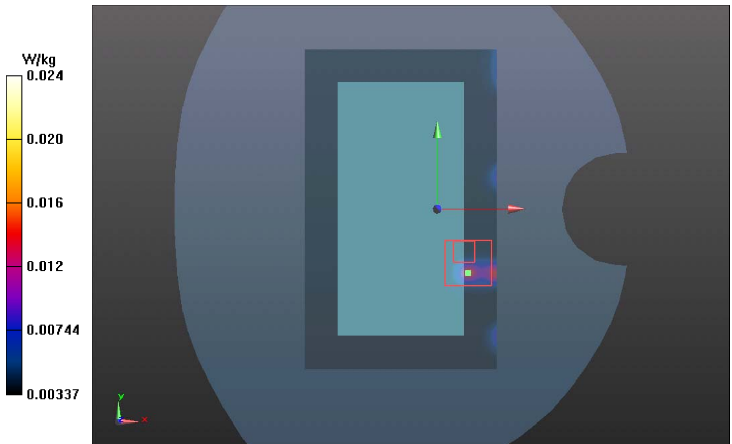
Figure 57 802.11a Test Position 1 Channel 44
