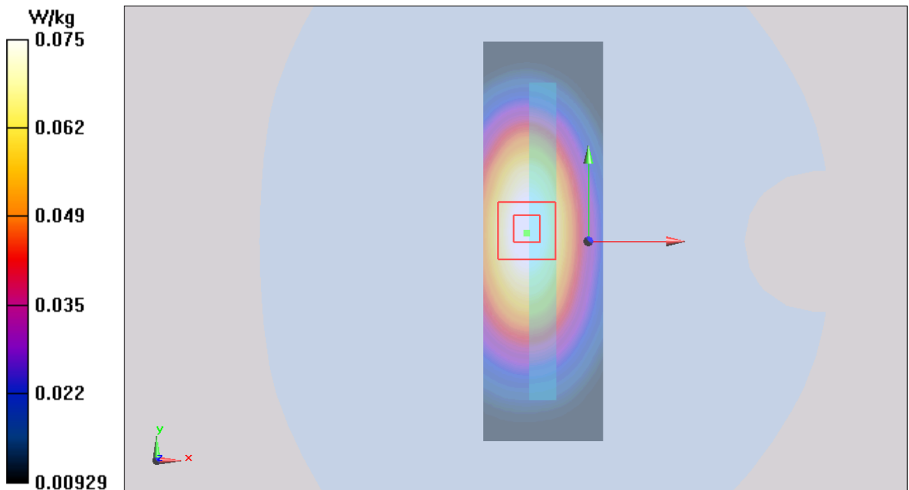
Figure 28 UMTS Band V with Test Position 5 Channel 4183
