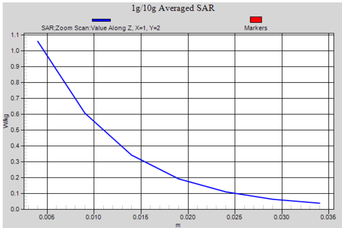
Figure 13 UMTS Band II with Test Position 1 Channel 9538
