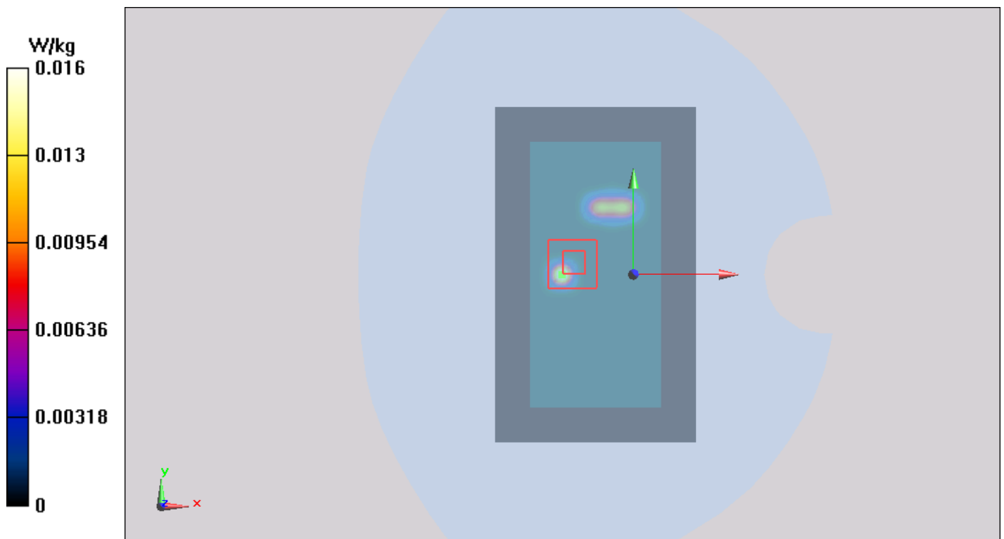
Figure 50 802.11a Test Position 2 Channel 56
