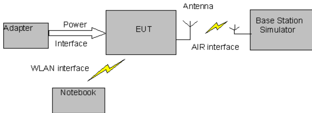
Connection Diagram (Mode 3~Mode 4)
