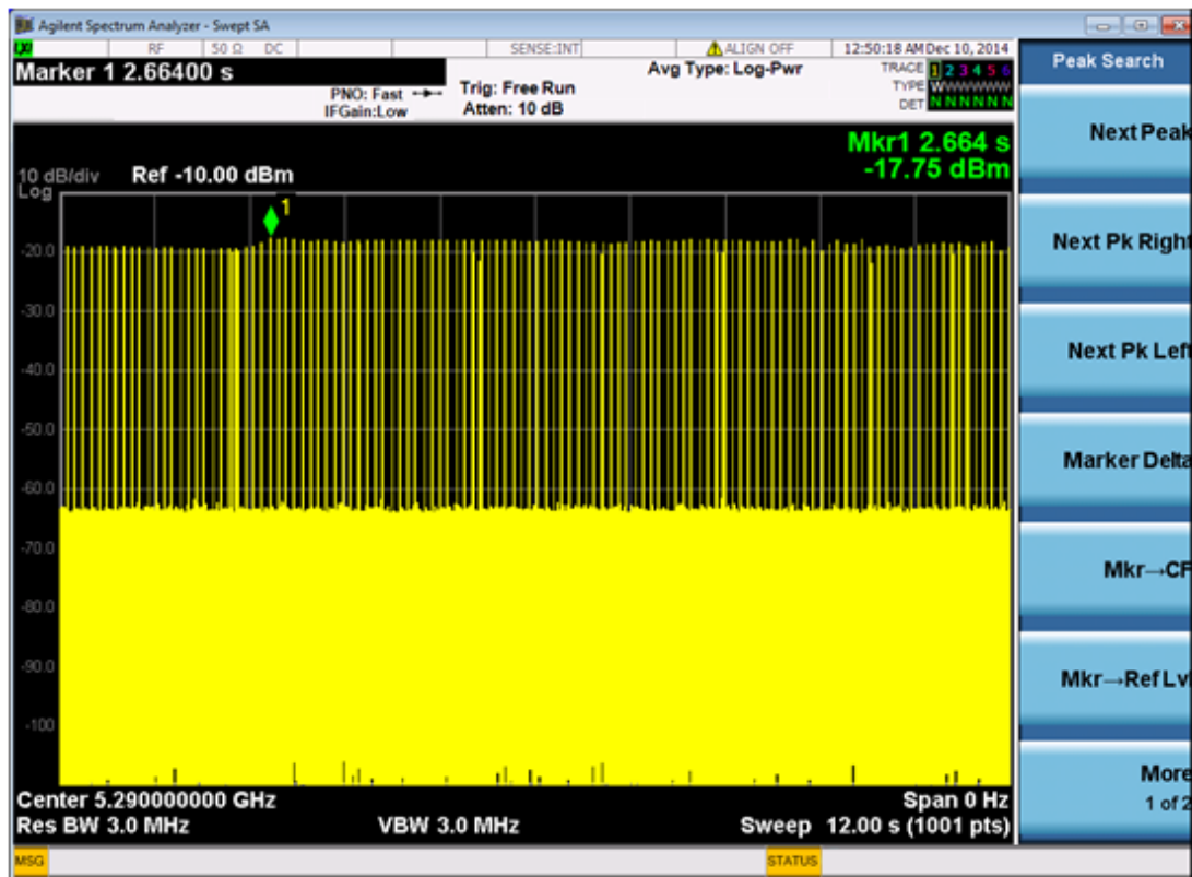
Calibration Radar Type 1 @ 5290MHz
