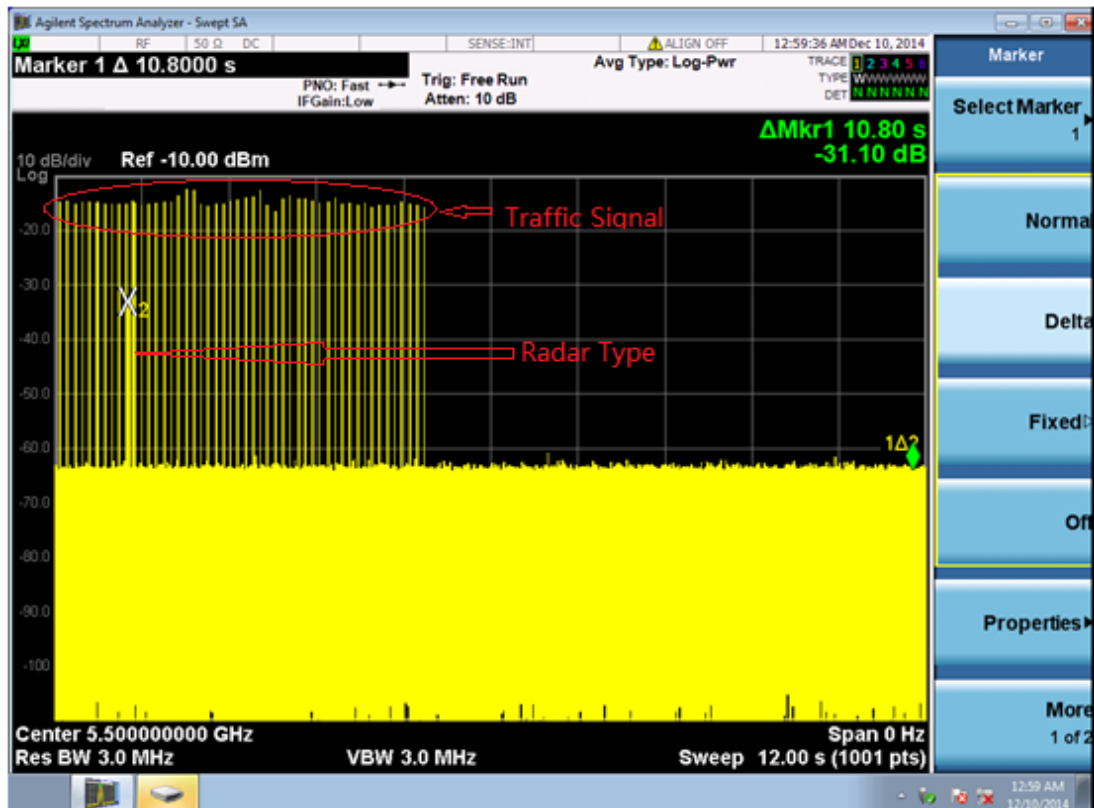
Channel Closing Transmission Time @ 5500MHz(Radar Type 1)
