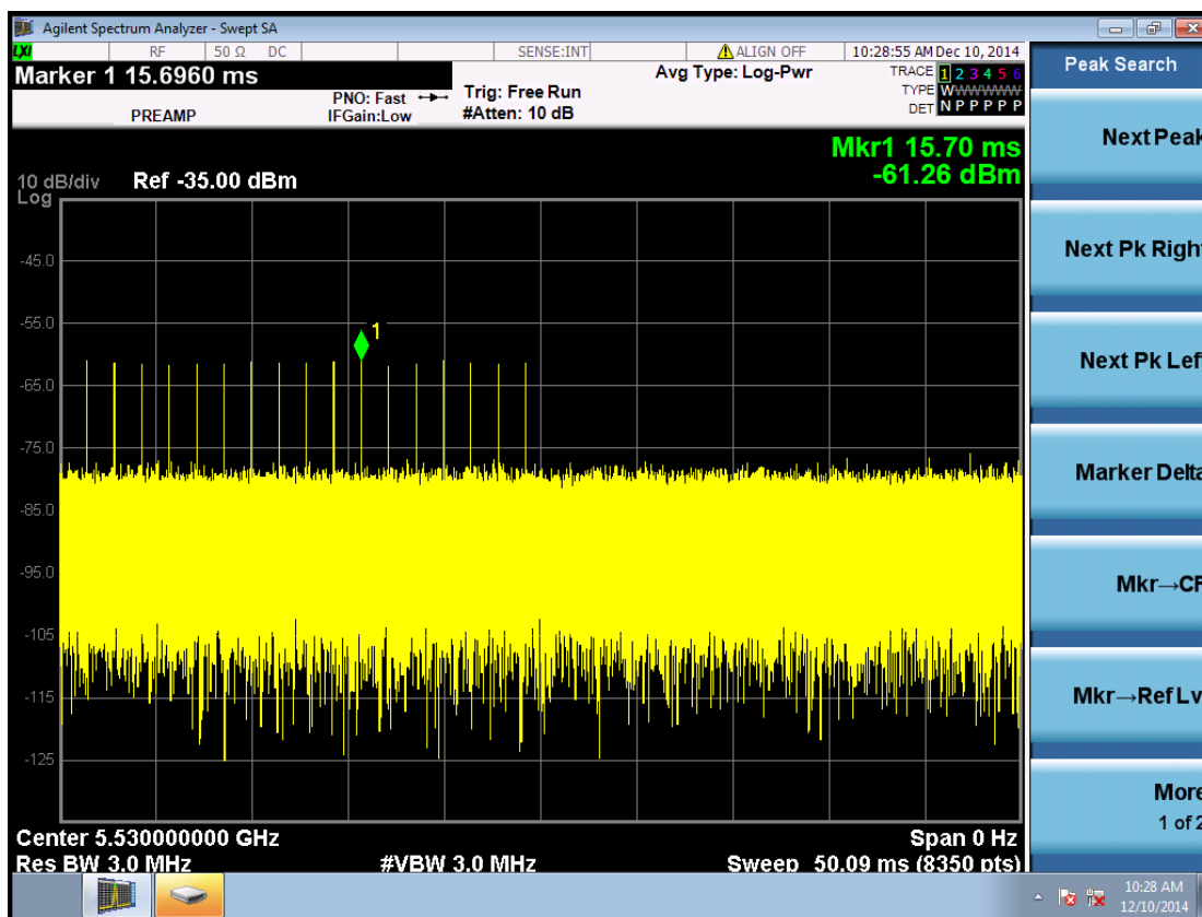
Calibration Radar Type 1 @ 5530MHz
