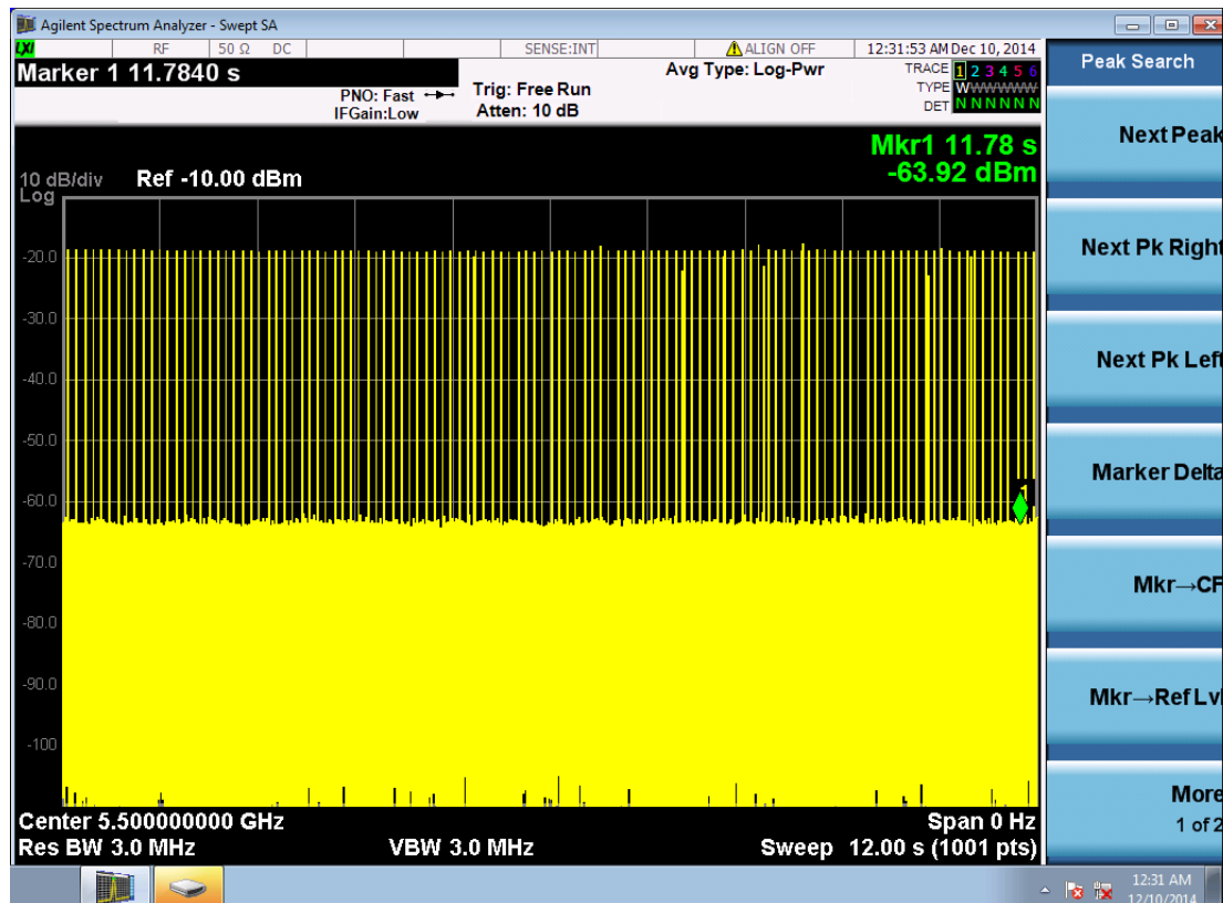
Calibration Radar Type 1 @ 5500MHz
