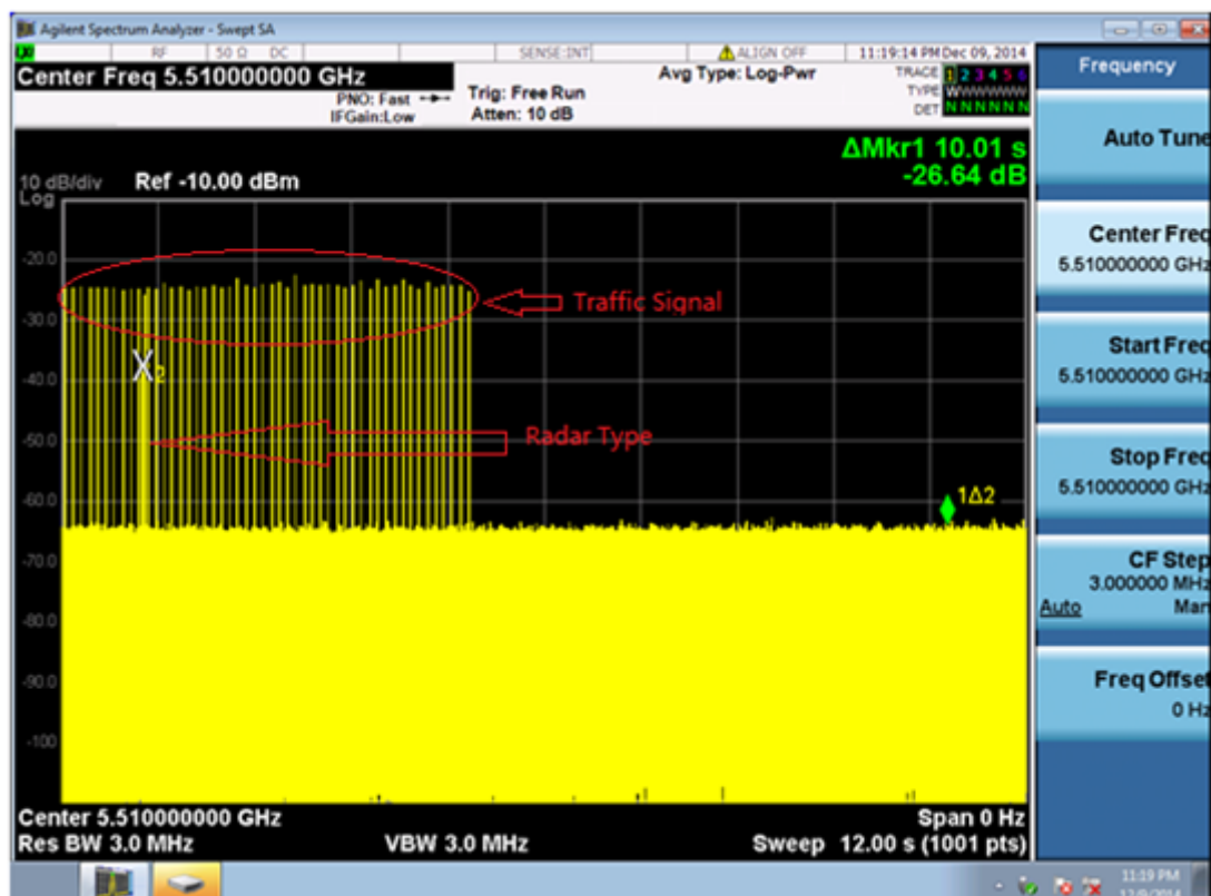
Channel Closing Transmission Time @ 5510MHz(Radar Type 1)
