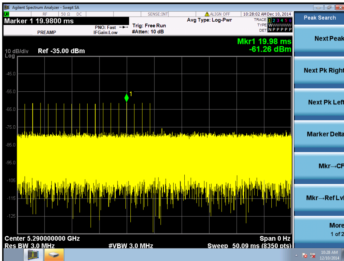
Calibration Radar Type 1 @ 5290MHz
