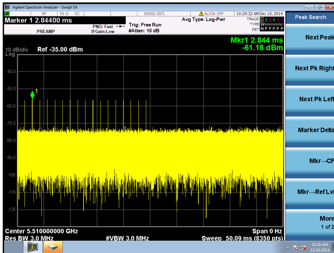
Calibration Radar Type 1 @ 5510MHz
