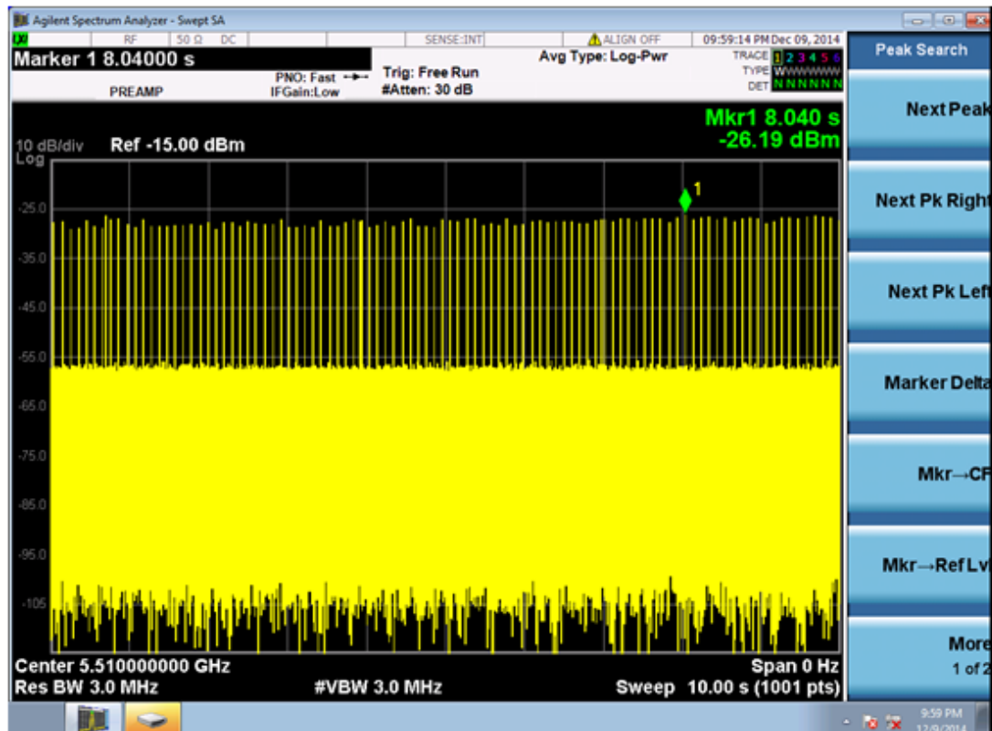
Calibration Radar Type 1 @ 5510MHz
