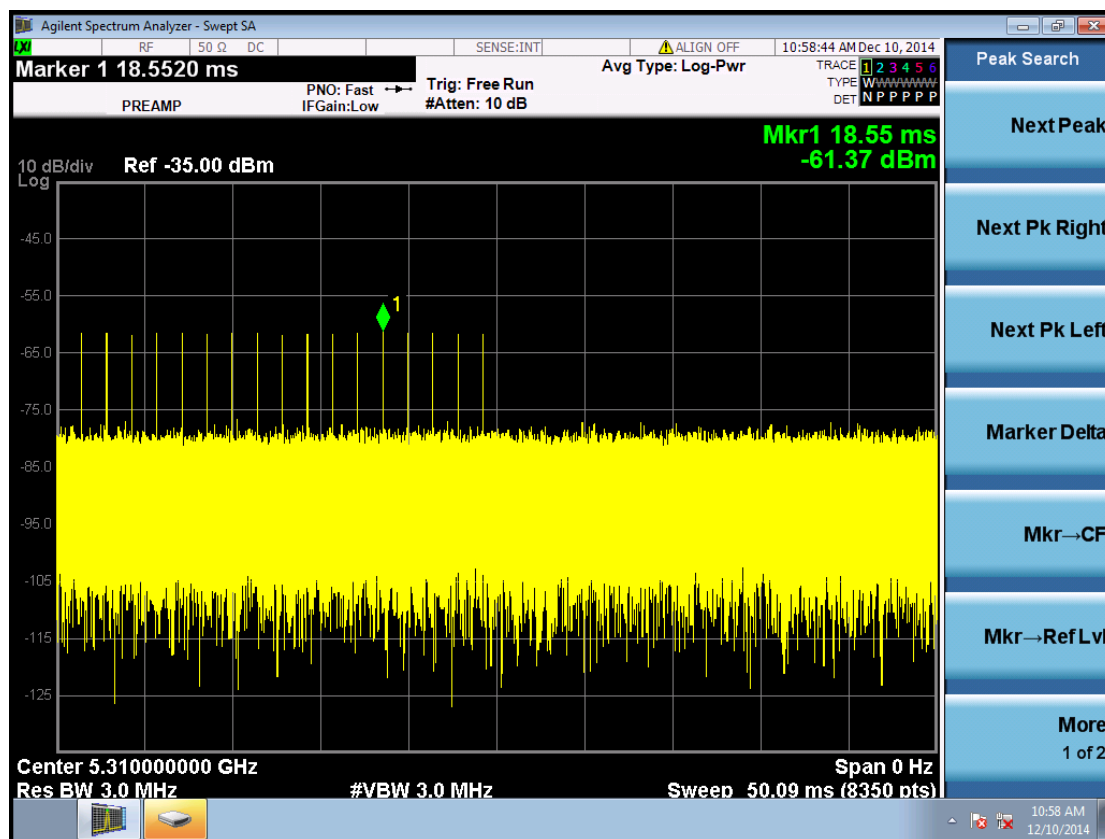
Calibration Radar Type 1 @ 5310MHz
