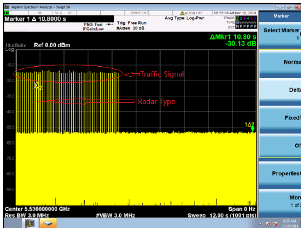
Channel Closing Transmission Time @ 5530MHz(Radar Type 1)
