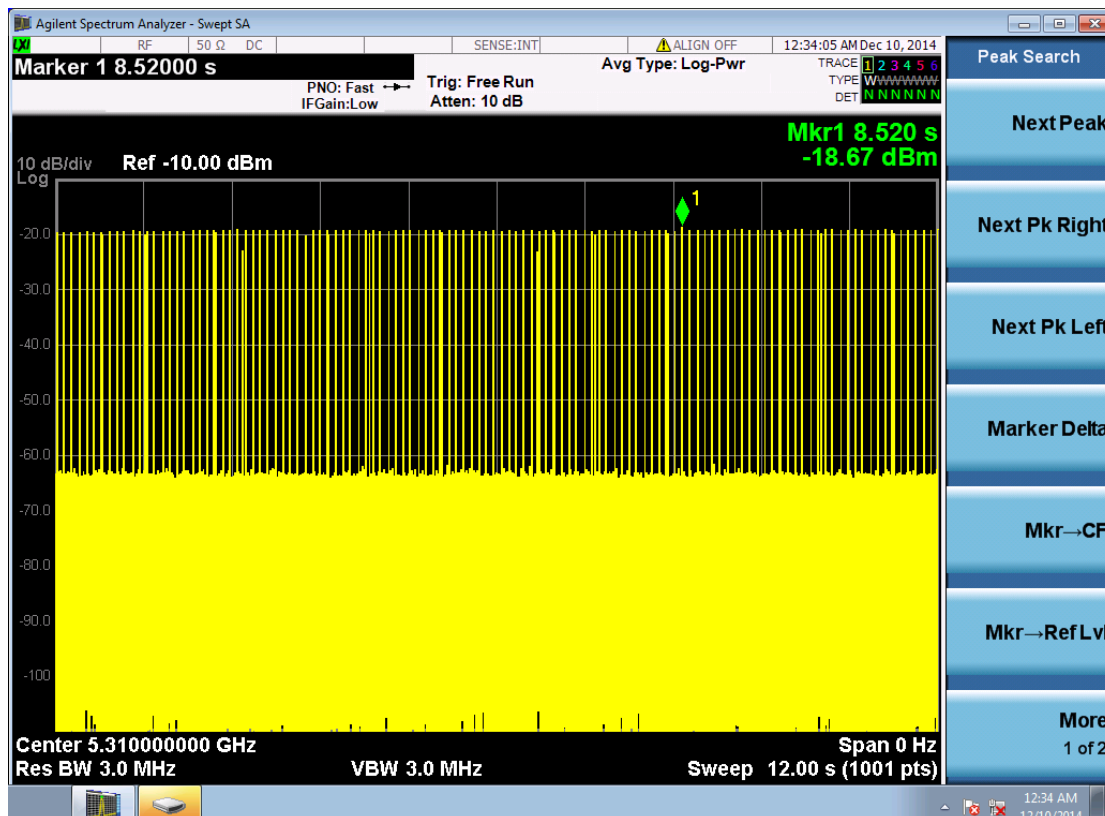
Calibration Radar Type 1 @ 5310MHz
