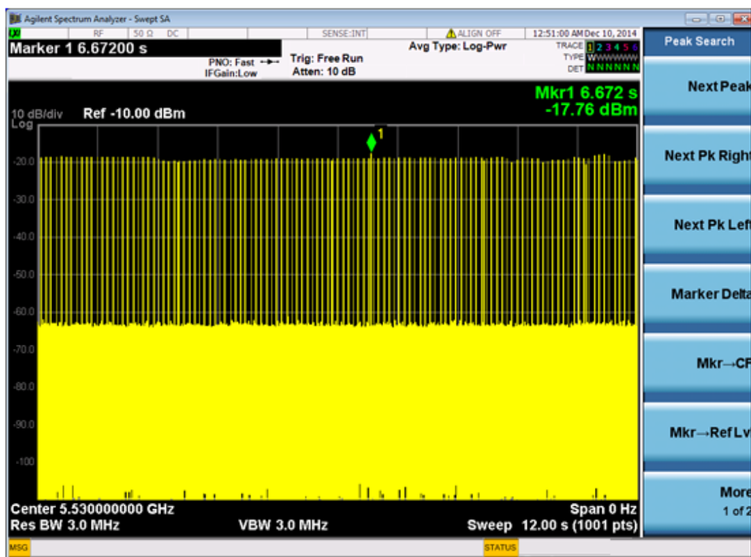
Calibration Radar Type 1 @ 5530MHz
