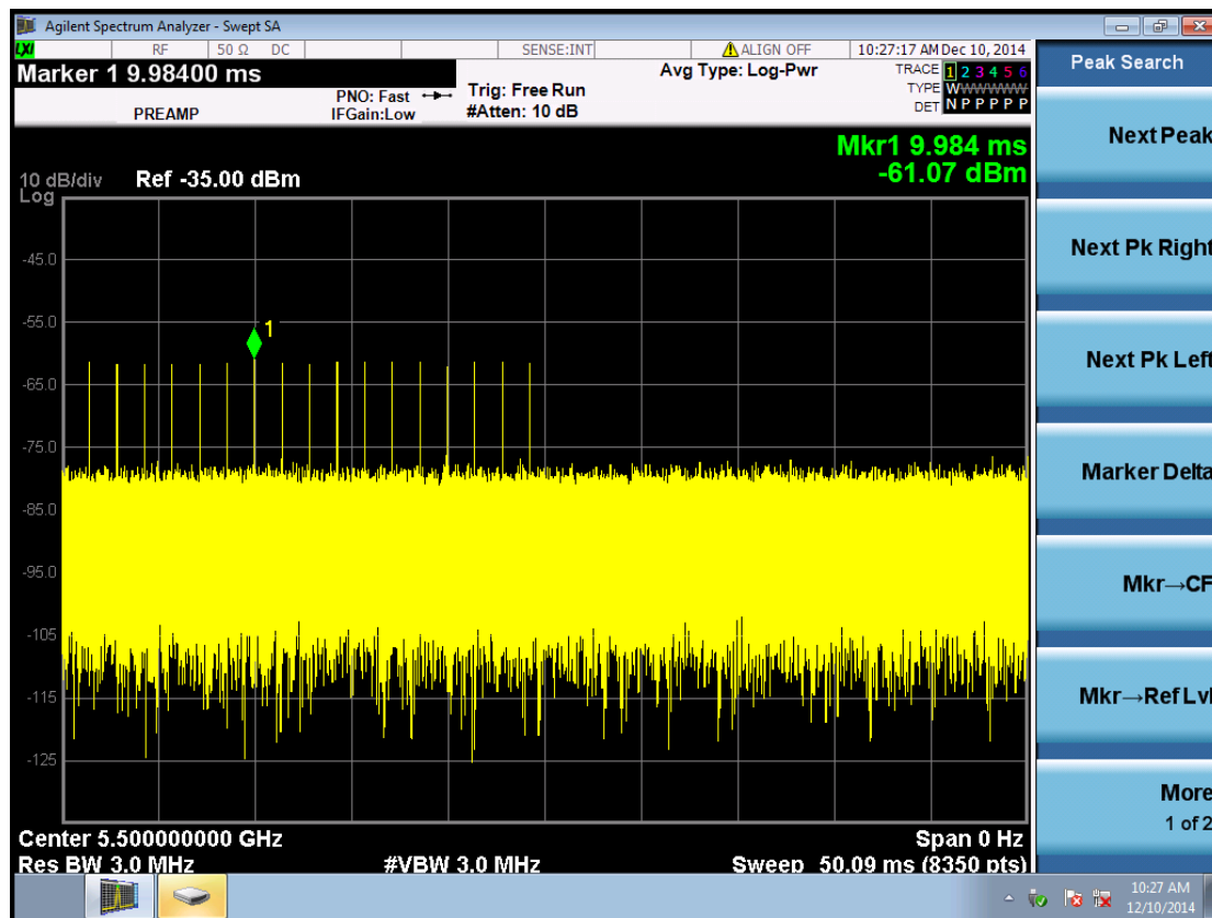
Calibration Radar Type 1 @ 5500MHz
