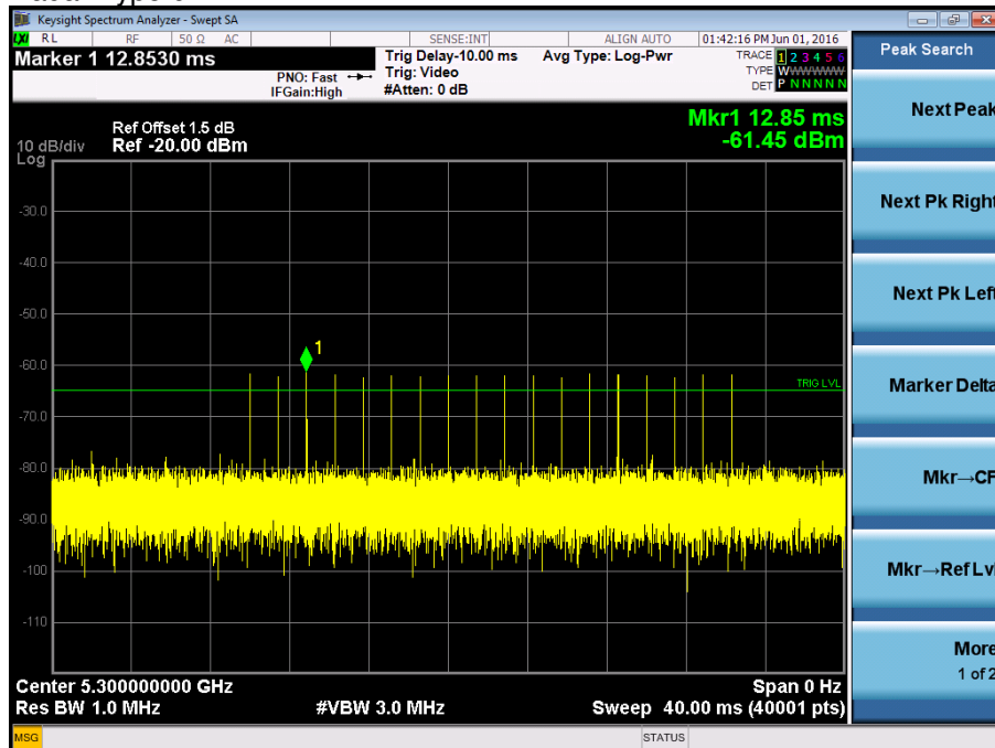
Radar Type 0
