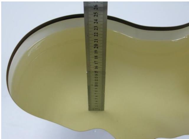
Photo 26: HSL2600MHz depth (15.0cm)
