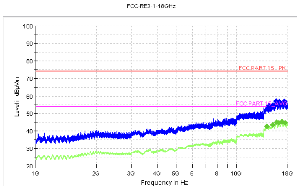
Figure A.13 Radiated Emission from 1GHz to 18GHz
