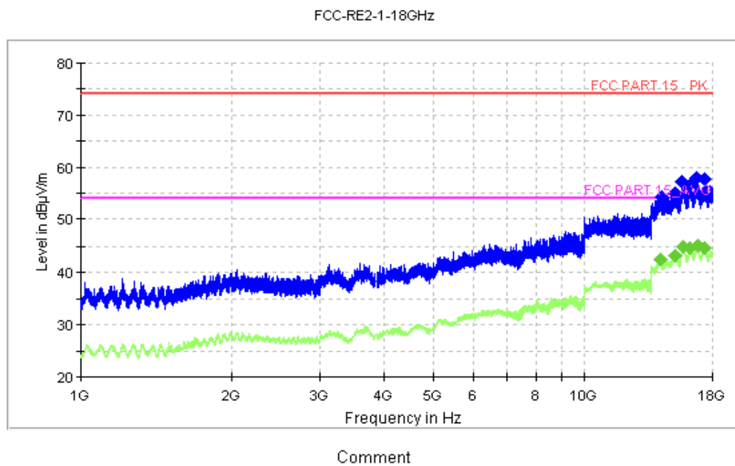
Figure A.9 Radiated Emission from 1GHz to 18GHz
