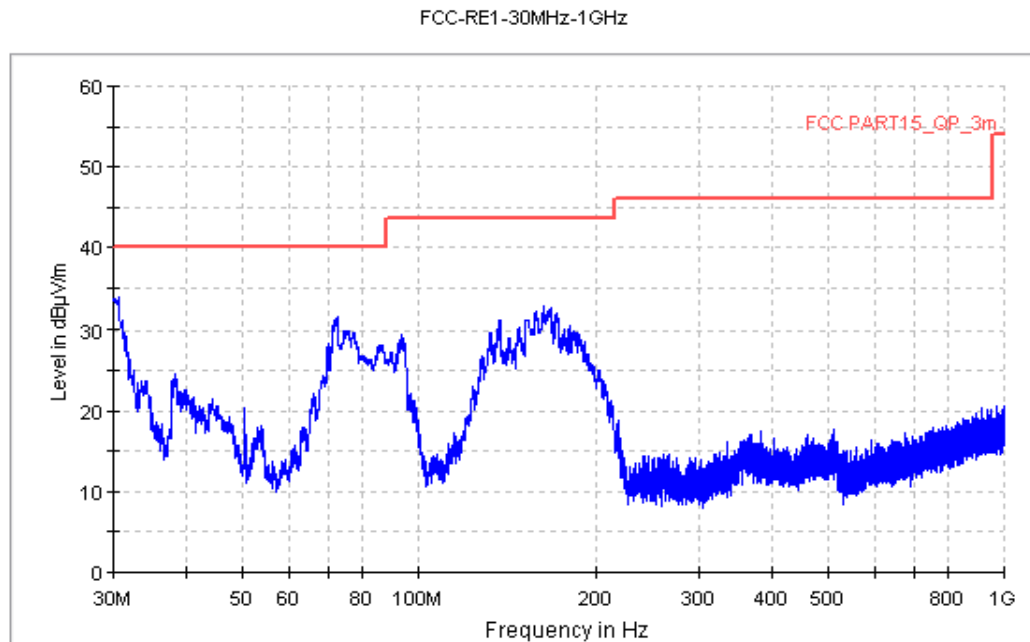
Figure A.12 Radiated Emission from 30MHz to 1GHz
