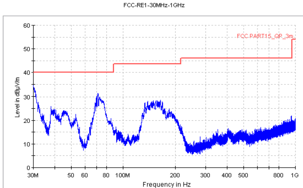
Figure A.10 Radiated Emission from 30MHz to 1GHz
