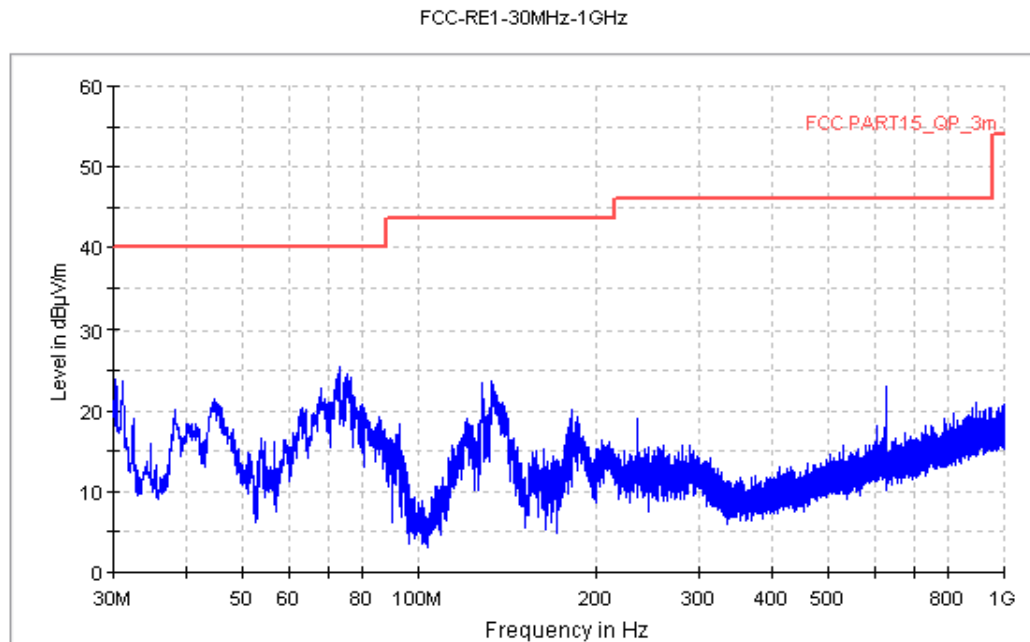
Figure A.8 Radiated Emission from 30MHz to 1GHz
