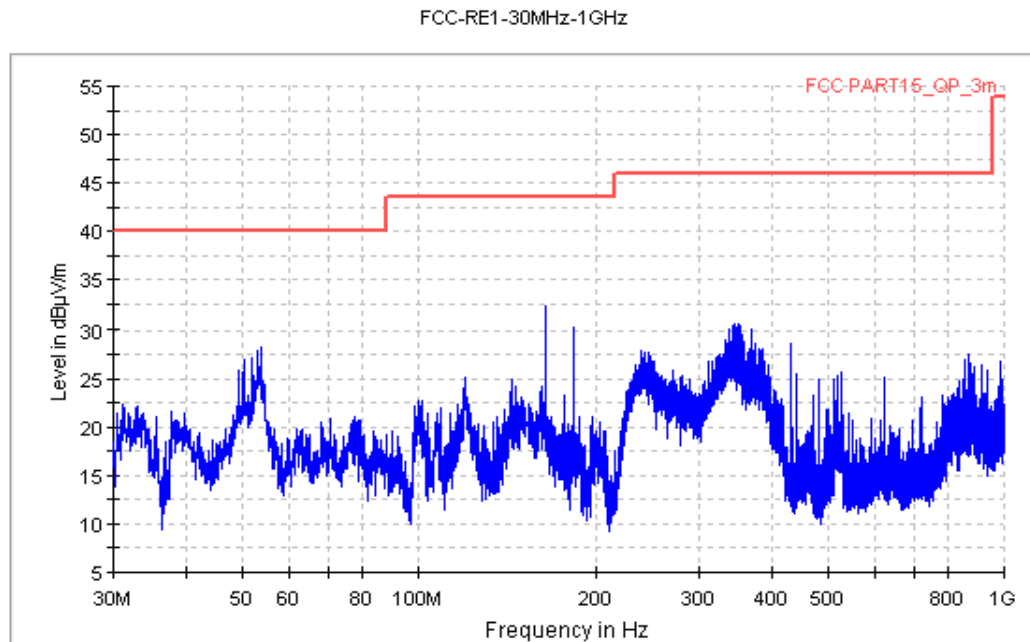
Figure A.14 Radiated Emission from 30MHz to 1GHz
