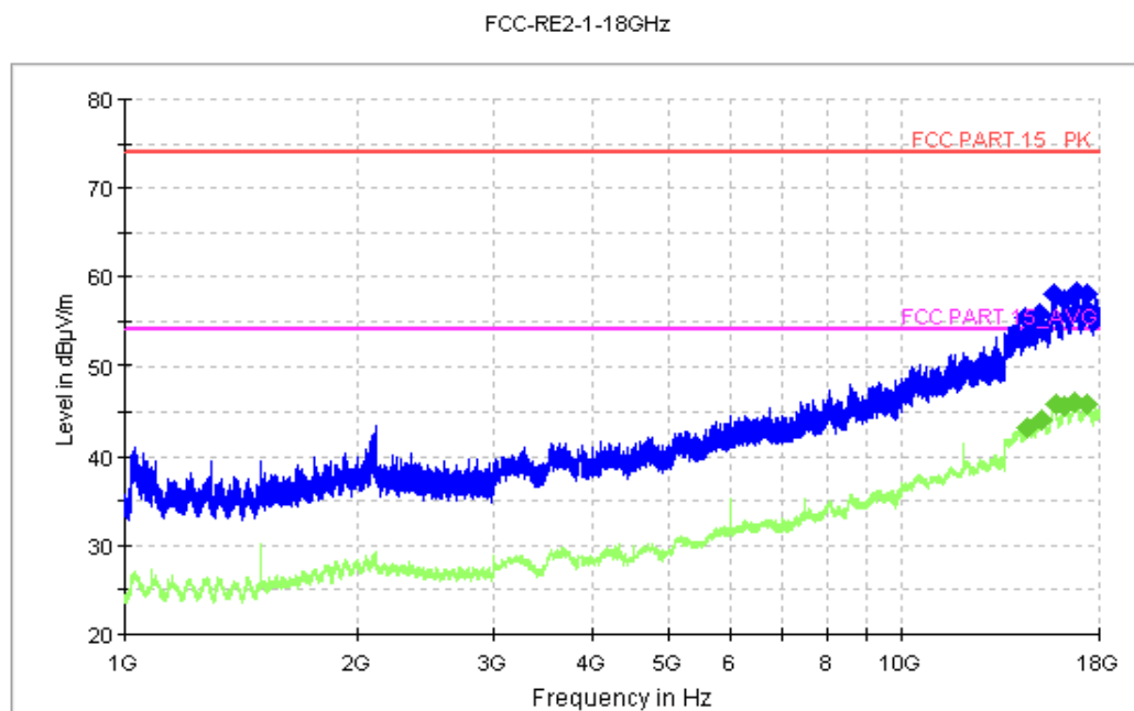
Figure A.15 Radiated Emission from 1GHz to 18GHz
