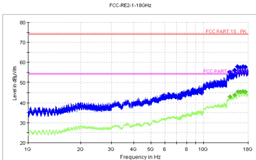
Figure A.7 Radiated Emission from 1GHz to 18GHz
