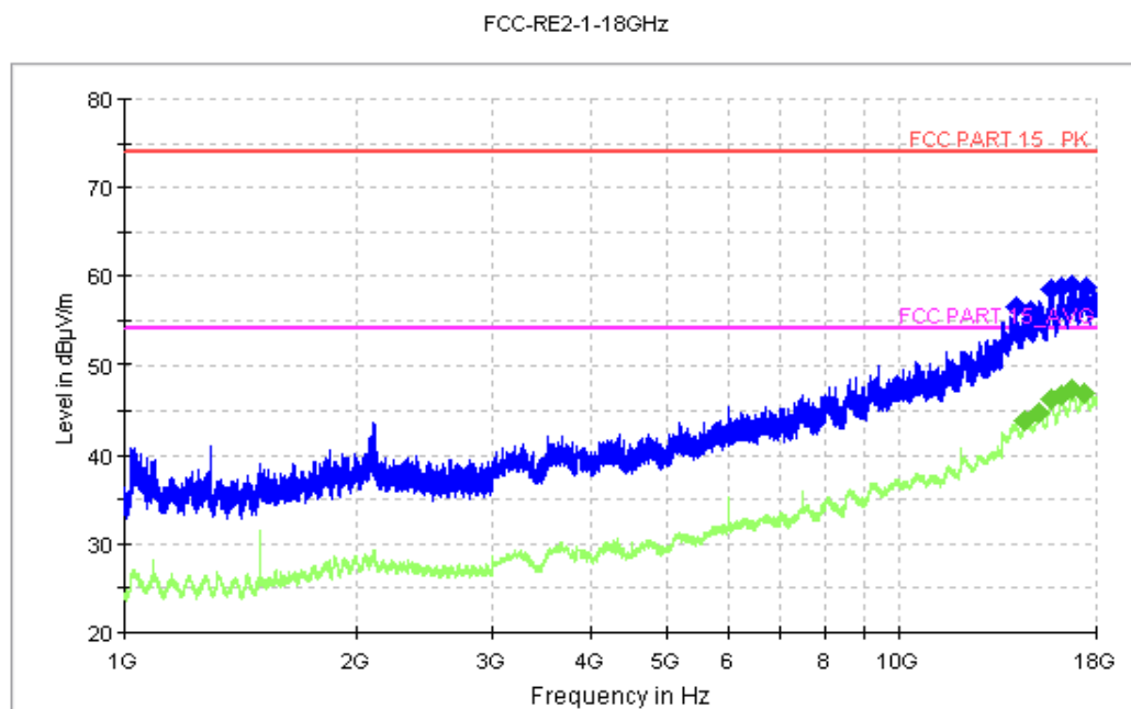
Figure A.17 Radiated Emission from 1GHz to 18GHz
