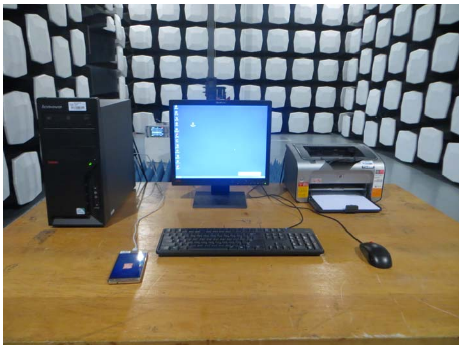
Picture 6: RE-USB(1GHz-18GHz)
