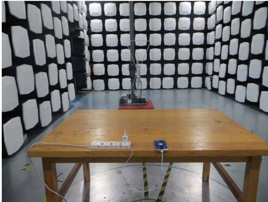
Picture 3: RE-Charging(30MHz-1GHz)
