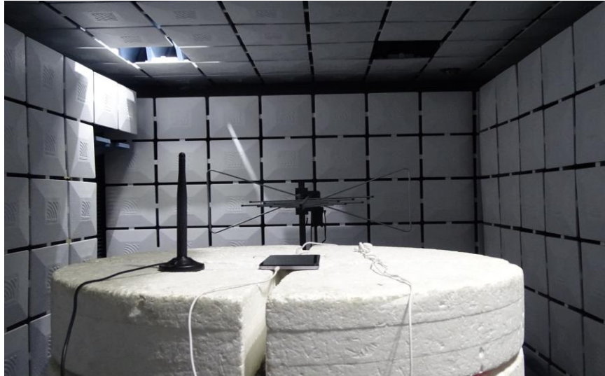
Radiated Spurious Emission (below 3GHz)
