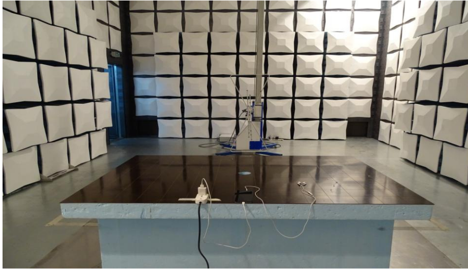
Radiated Spurious Emission (below 1GHz)
