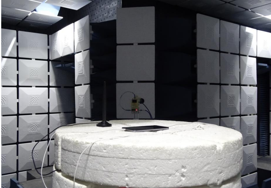
Radiated Spurious Emission (18GHz to26.5GHz)
