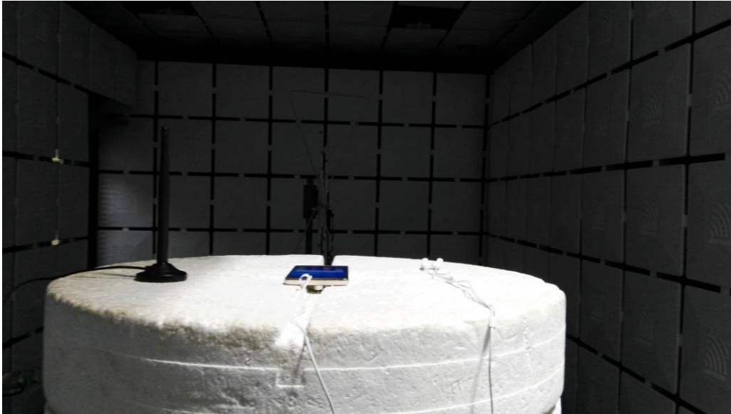
Radiated Spurious Emission (below 1GHz)
