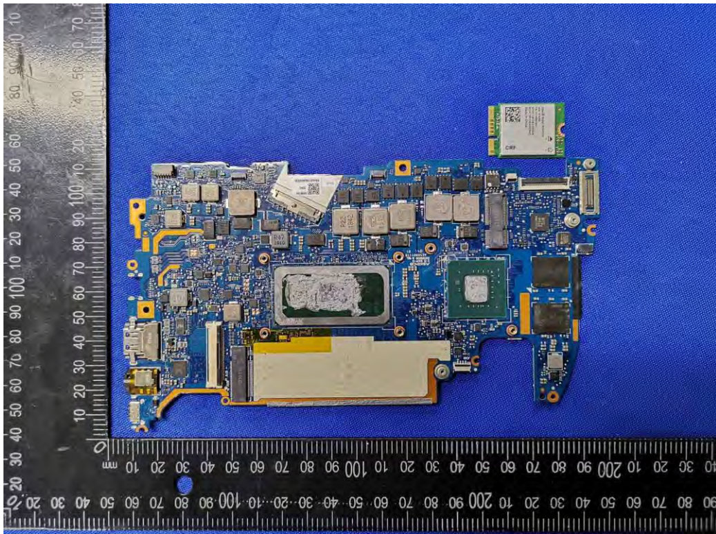
MAIN BOARD TOP VIEW-WITH GPU VERSION
