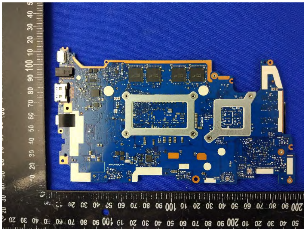
MAIN BOARD REAR VIEW- WITHOUT GPU VERSION
