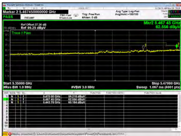
Band III 11ac160 CH114
