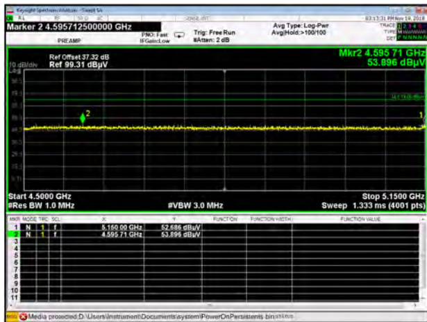
Band I 11ac20 CH36
