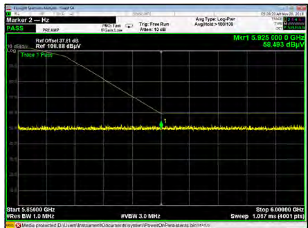
Band IV 11ac20 CH165
