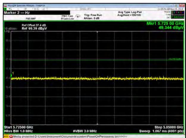
Band III 11ac40 CH134
