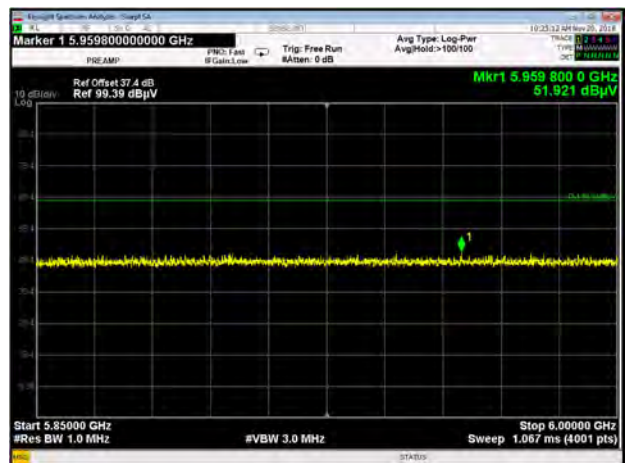
Band III 11ac80 CH138
