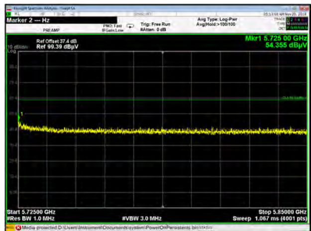
Band III 11ac20 CH140
