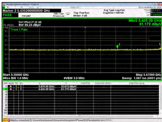
Band III 11ac20 CH100
