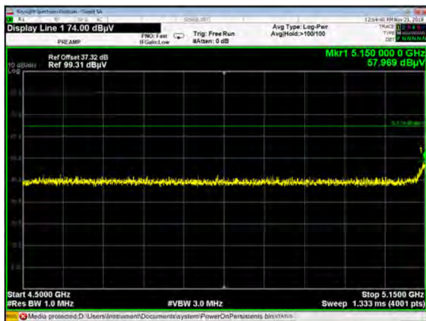
Band I 11ac40 CH38
