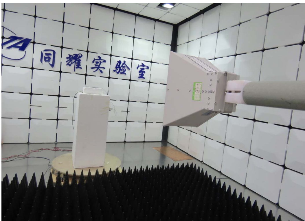
Above 1GHz
