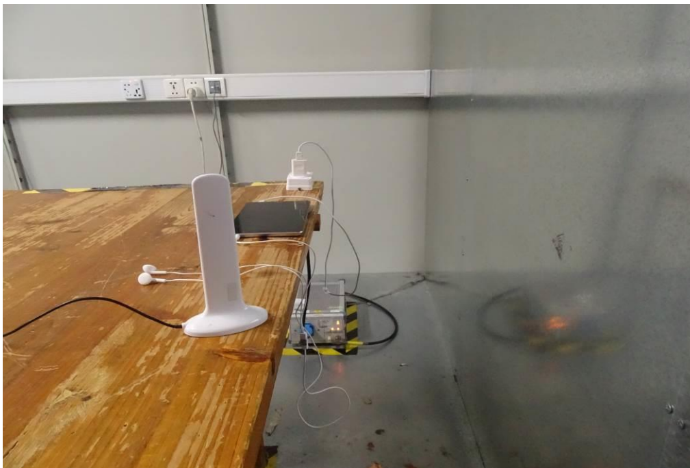
Conducted Emissions with AC Ports
