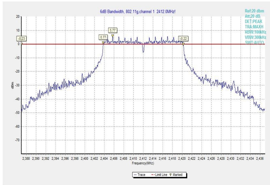
Fig.13 Occupied 6dB Bandwidth (802.11g, Ch 1)
