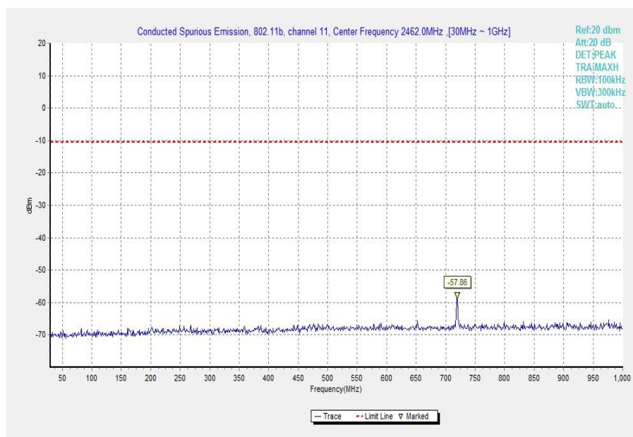
Fig.32 Conducted Spurious Emission (802.11b, Ch11, 30 MHz-1 GHz)
