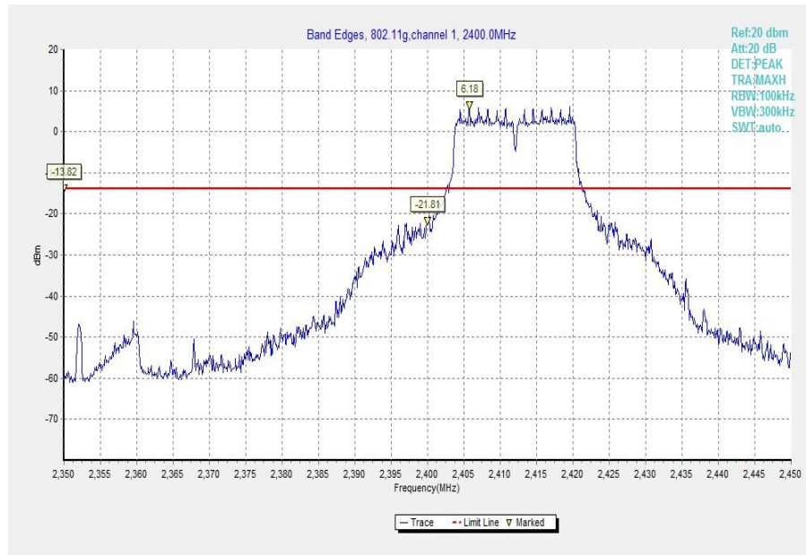
Fig.21 Band Edges (802.11g, Ch 1)
