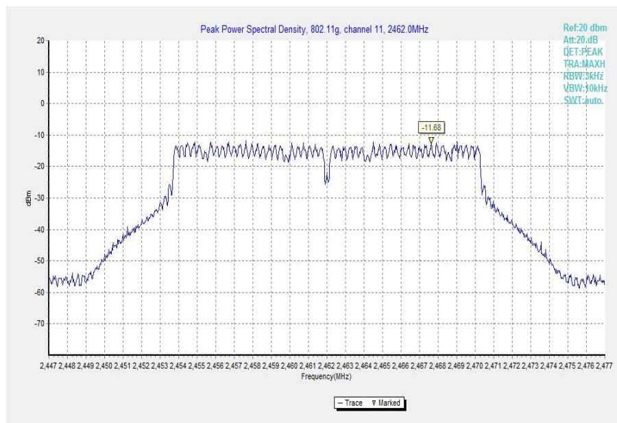
Fig.6 Power Spectral Density (802.11g, Ch 11)
