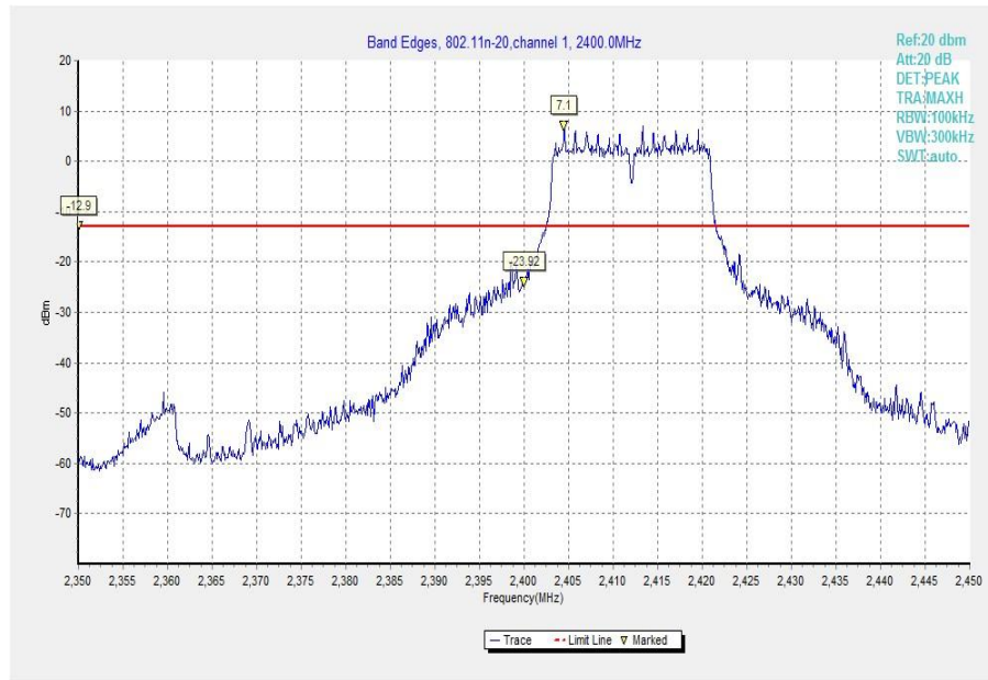
Fig.23 Band Edges (802.11 n-20MHz, Ch 1)
