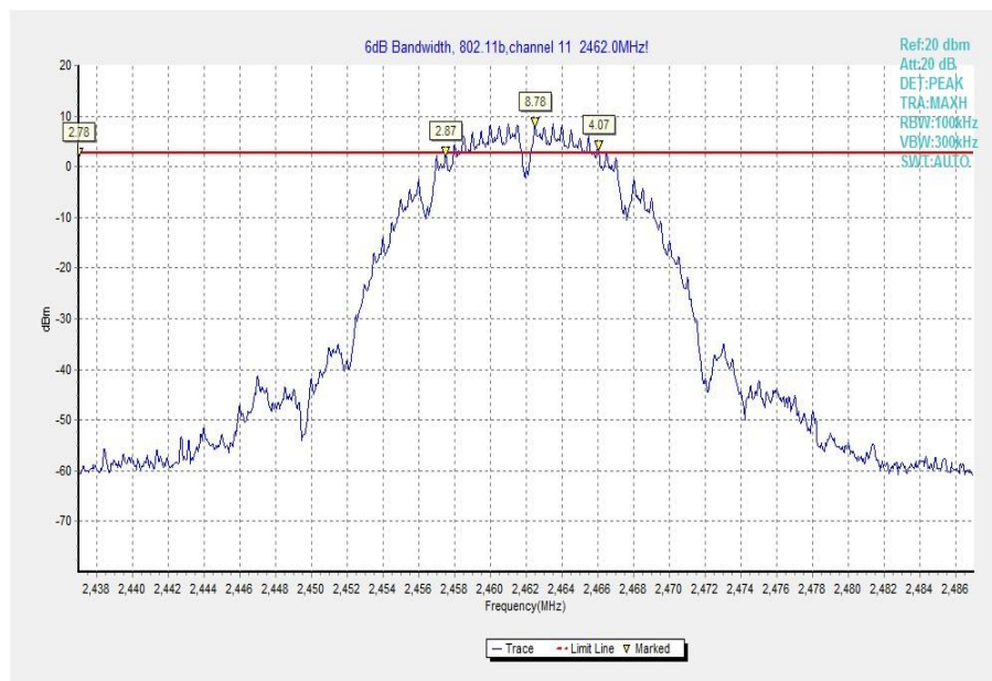
Fig.12 Occupied 6dB Bandwidth (802.11b, Ch 11)
