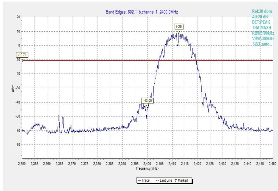
Fig.19 Band Edges (802.11b, Ch 1)
