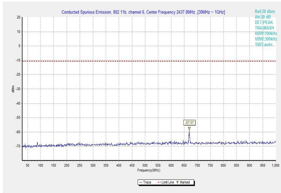
Fig.29 Conducted Spurious Emission (802.11b, Ch6, 30 MHz-1 GHz)
