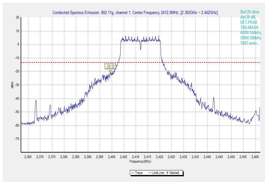
Fig.34 Conducted Spurious Emission (802.11g, Ch1, Center Frequency)
