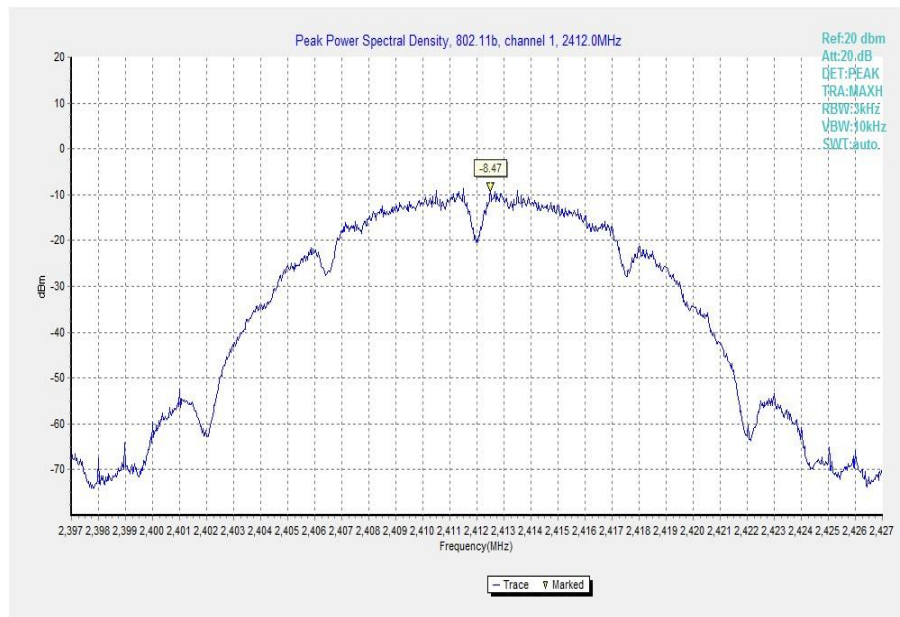
Fig.1 Power Spectral Density (802.11b, Ch 1)
