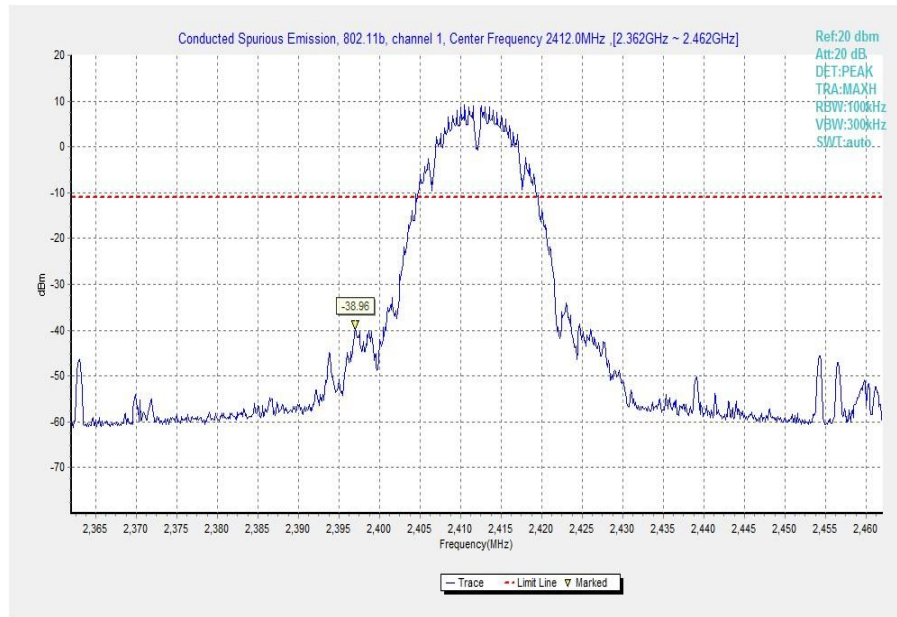
Fig.25 Conducted Spurious Emission (802.11b, Ch1, Center Frequency)
