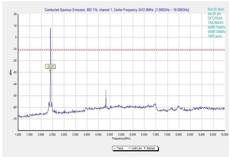
Fig.27 Conducted Spurious Emission (802.11b, Ch1, 1 GHz-10 GHz)
