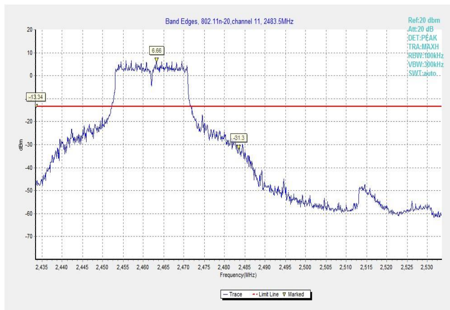
Fig.24 Band Edges (802.11 n-20MHz, Ch 11)
