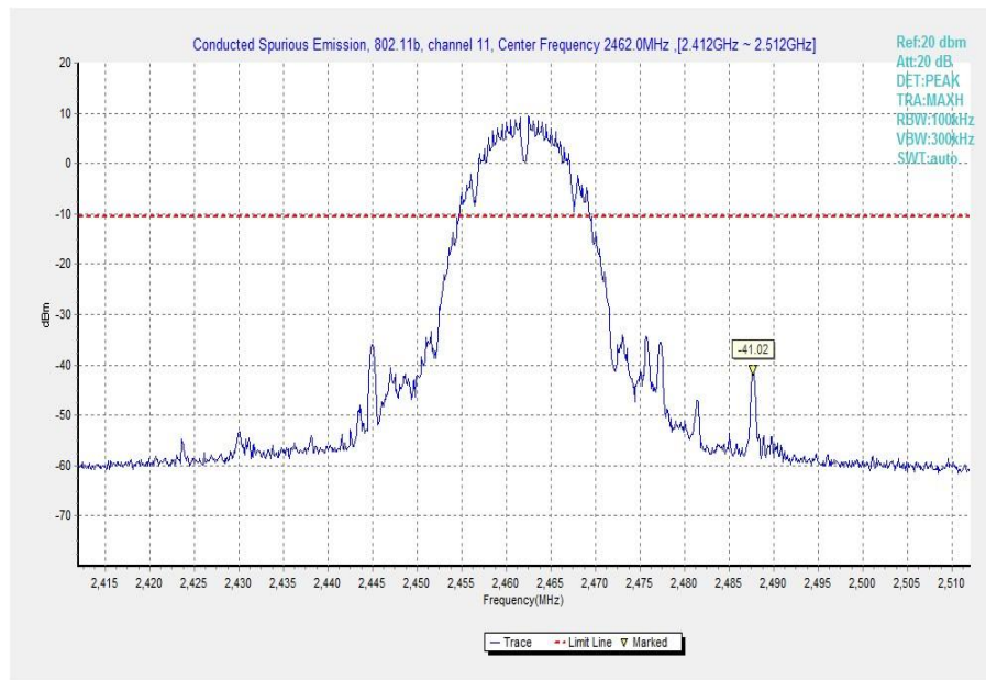
Fig.31 Conducted Spurious Emission (802.11b, Ch11, Center Frequency)
