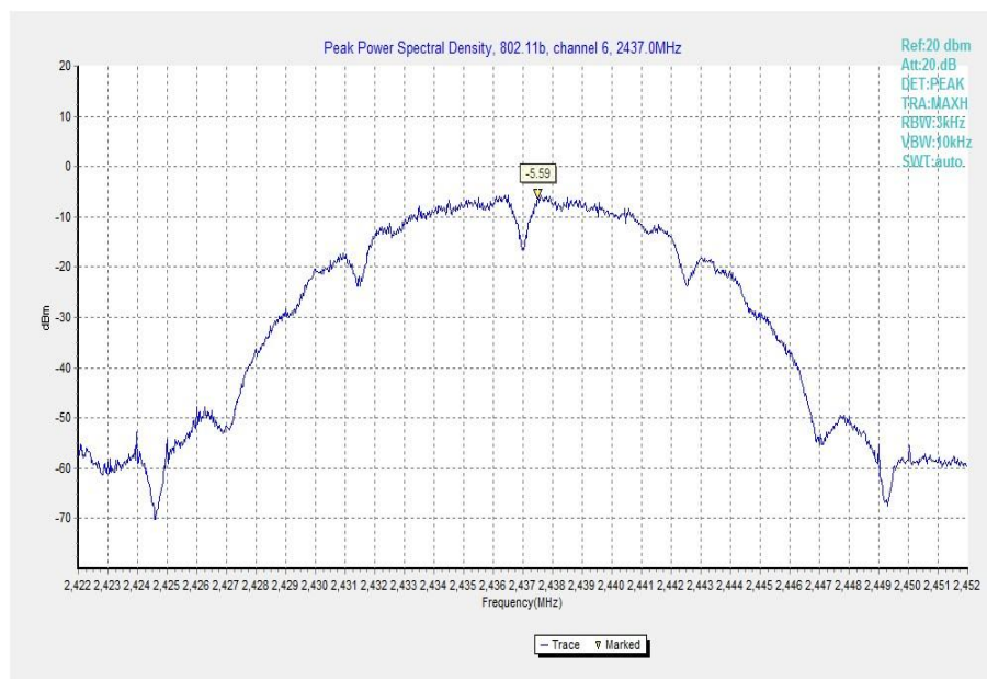
Fig.2 Power Spectral Density (802.11b, Ch 6)
