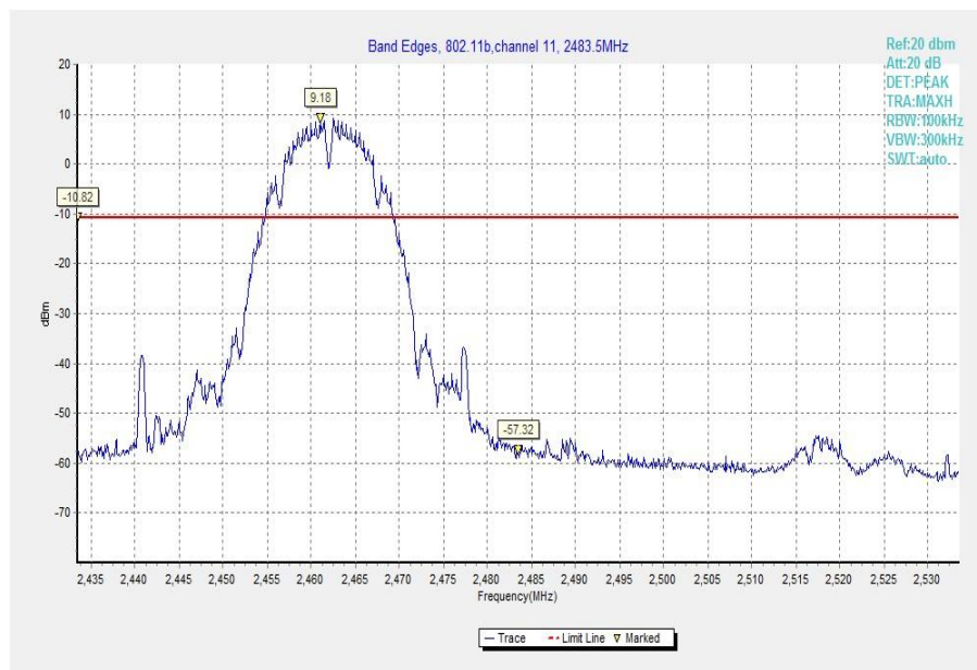
Fig.20 Band Edges (802.11b, Ch 11)
