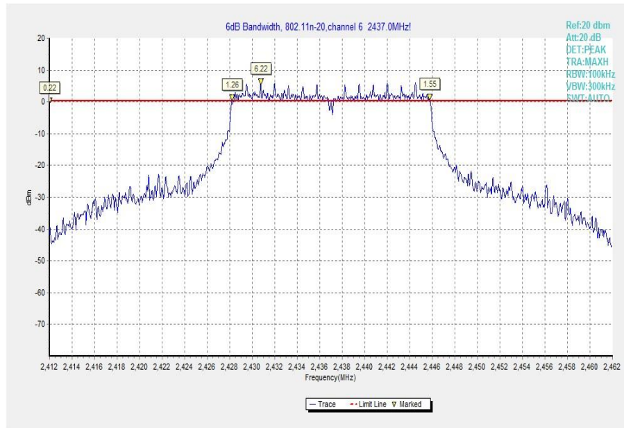
Fig.17 Occupied 6dB Bandwidth (802.11 n-20MHz, Ch 6)
