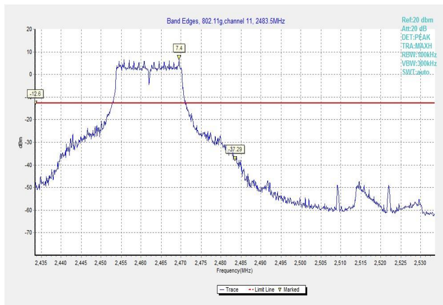
Fig.22 Band Edges (802.11g, Ch 11)
