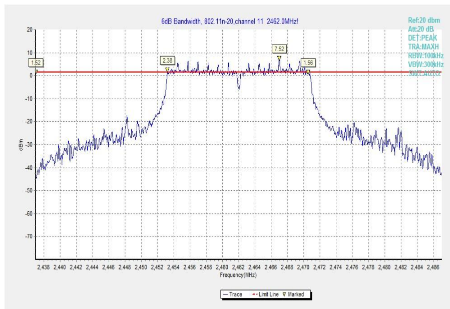
Fig.18 Occupied 6dB Bandwidth (802.11 n-20MHz, Ch 11)
