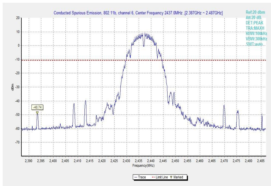
Fig.28 Conducted Spurious Emission (802.11b, Ch6, Center Frequency)
