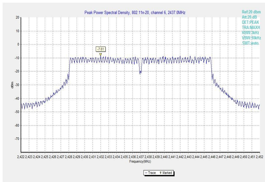
Fig.8 Power Spectral Density (802.11n-20MHz, Ch 6)
