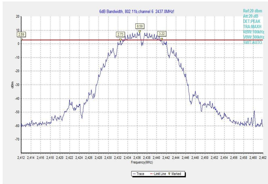
Fig.11 Occupied 6dB Bandwidth (802.11b, Ch 6)
