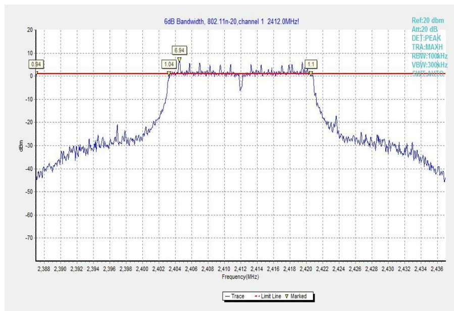
Fig.16 Occupied 6dB Bandwidth (802.11 n-20MHz, Ch 1)
