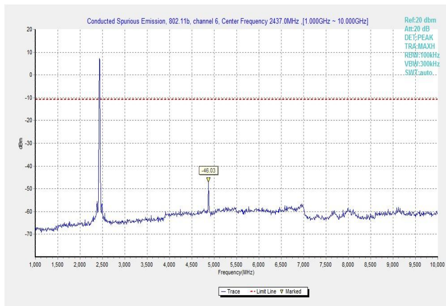
Fig.30 Conducted Spurious Emission (802.11b, Ch6, 1 GHz-10 GHz)
