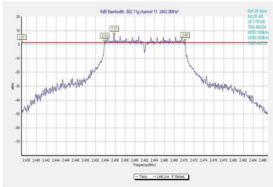
Fig.15 Occupied 6dB Bandwidth (802.11g, Ch 11)
