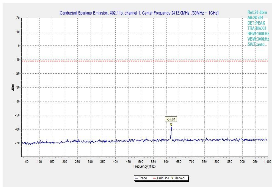
Fig.26 Conducted Spurious Emission (802.11b, Ch1, 30 MHz-1 GHz)
