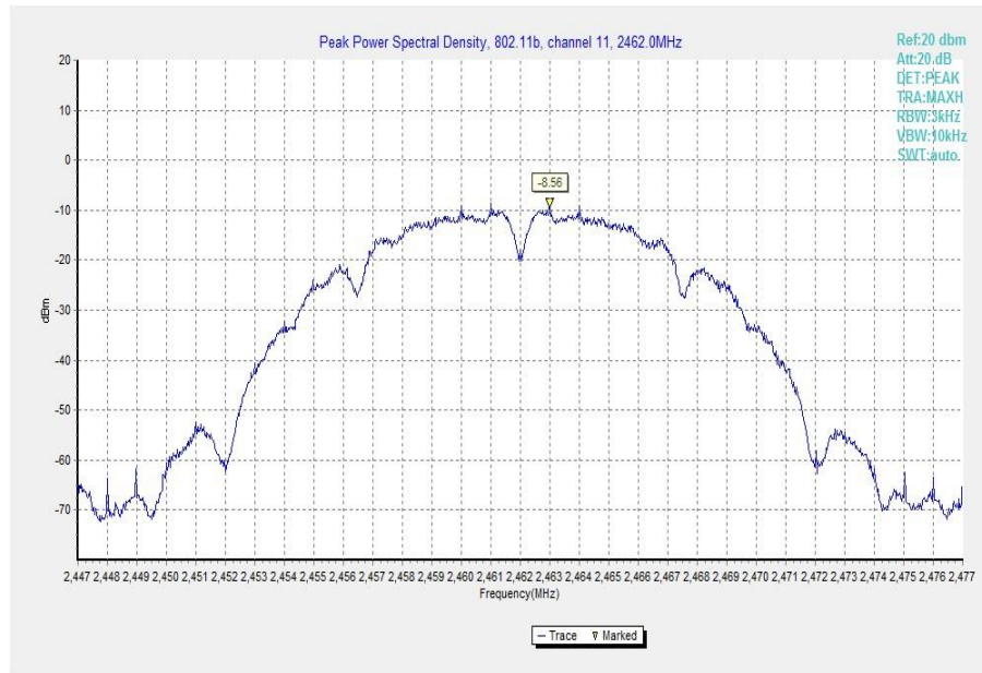
Fig.3 Power Spectral Density (802.11b, Ch 11)
