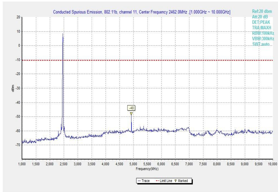
Fig.33 Conducted Spurious Emission (802.11b, Ch11, 1 GHz-10 GHz)
