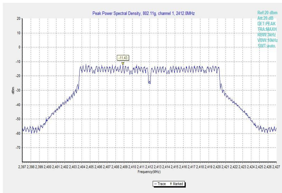
Fig.4 Power Spectral Density (802.11g, Ch 1)
