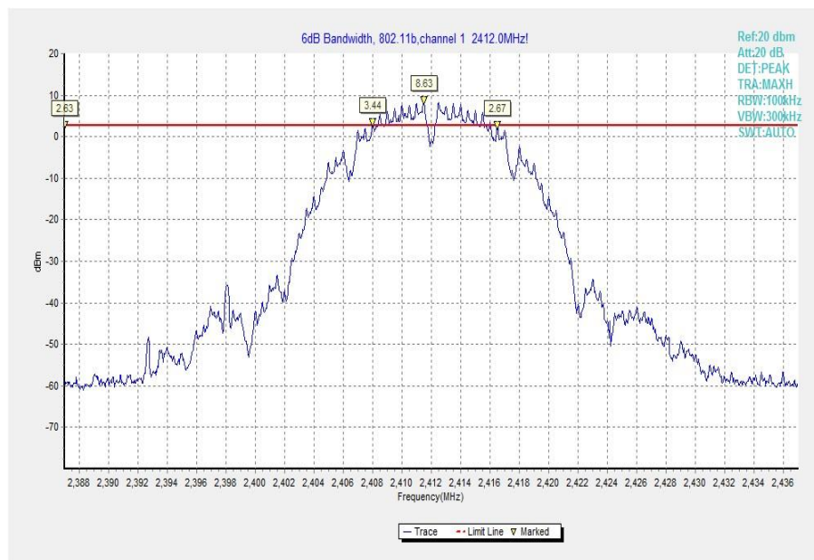
Fig.10 Occupied 6dB Bandwidth (802.11b, Ch 1)
