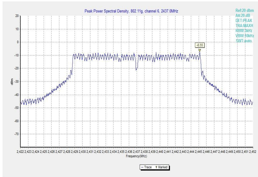
Fig.5 Power Spectral Density (802.11g, Ch 6)
