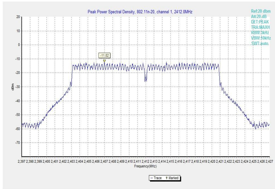
Fig.7 Power Spectral Density (802.11n-20MHz, Ch 1)
