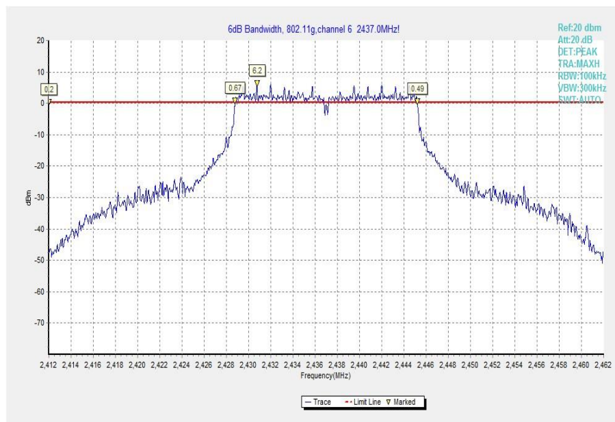
Fig.14 Occupied 6dB Bandwidth (802.11g, Ch 6)
