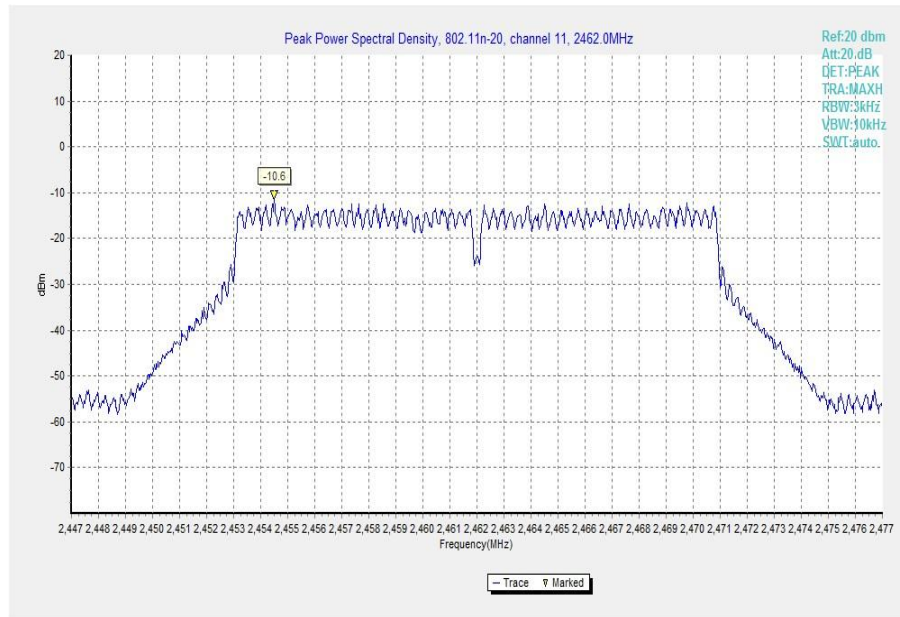
Fig.9 Power Spectral Density (802.11n-20MHz, Ch 11)
