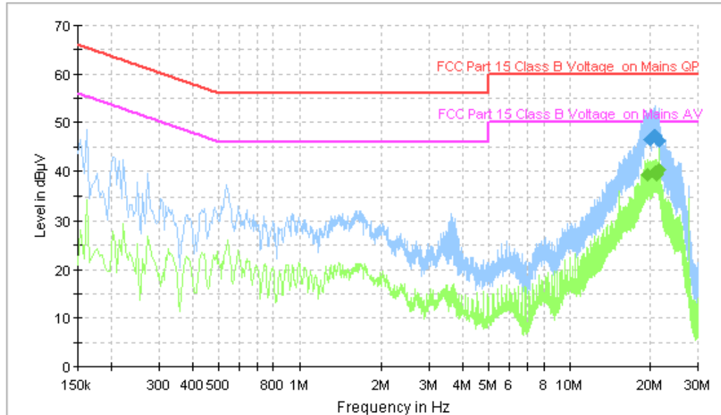
Figure A.31 Conducted Emission
