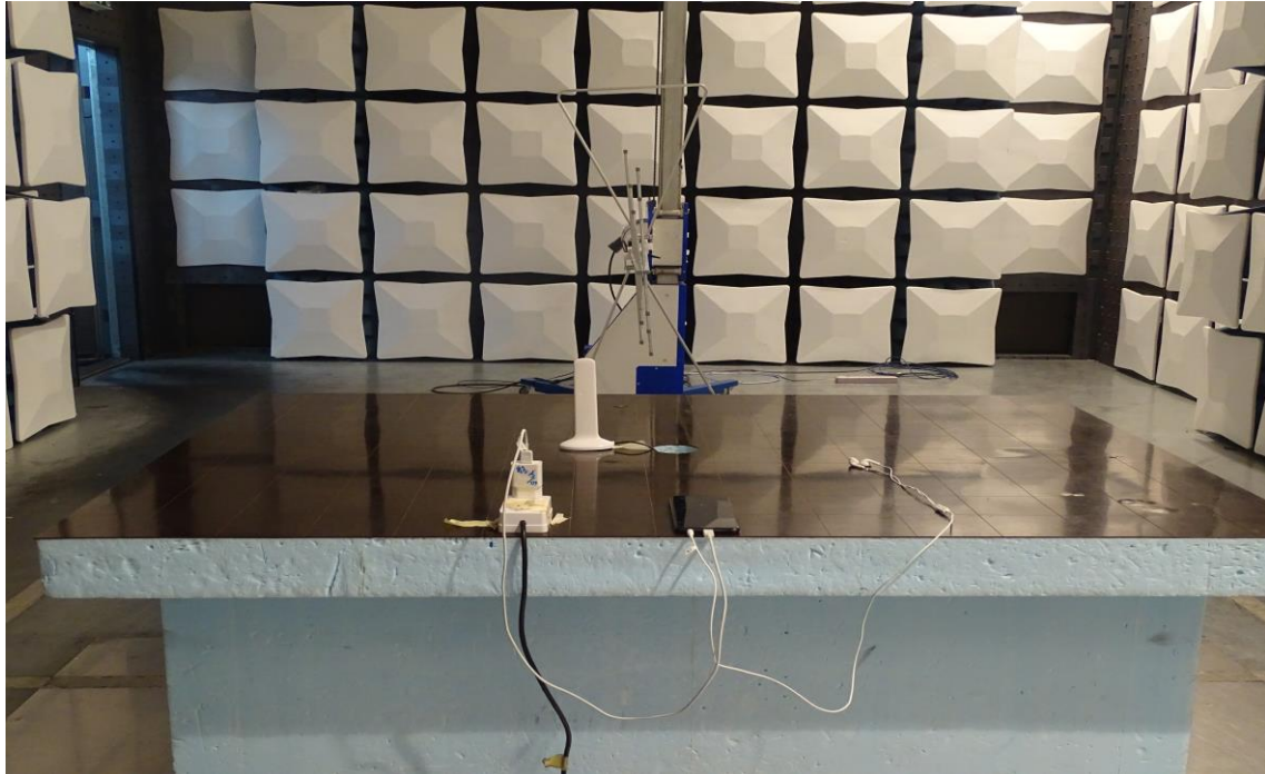
Radiated Disturbance Emissions (below 1GHz)
