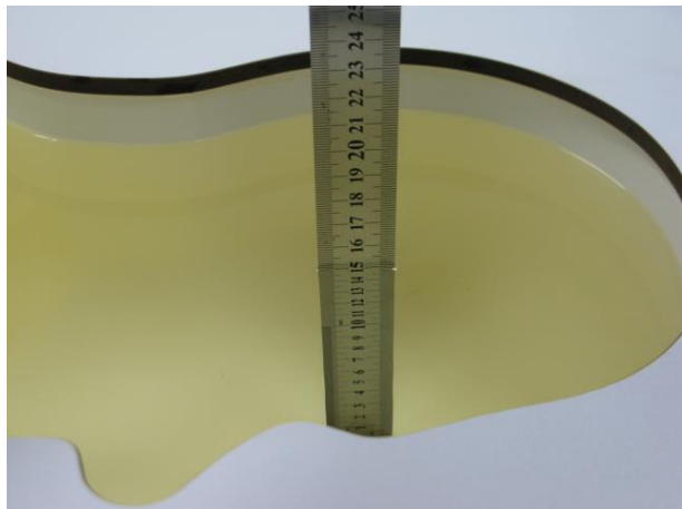
Photo 6: HSL2450MHz Depth (15.2cm)
