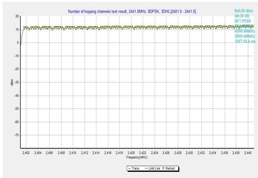
Fig. 93 Hopping channel ch0~39 (8DPSK, Ch39)
