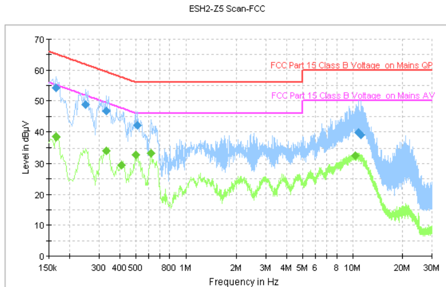
Fig. 101 AC Power line Conducted Emission (Idle, AE2)
