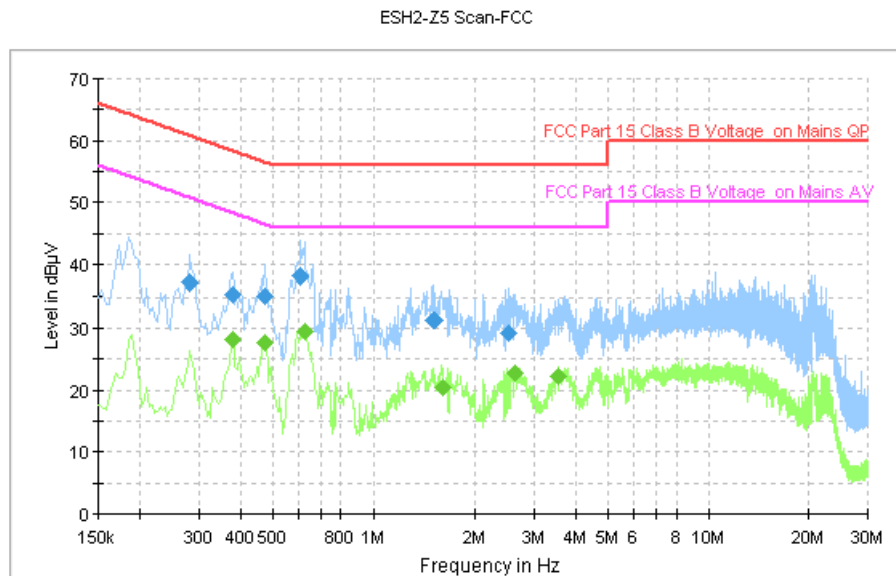
Fig. 103 AC Power line Conducted Emission (Idle, AE3)
