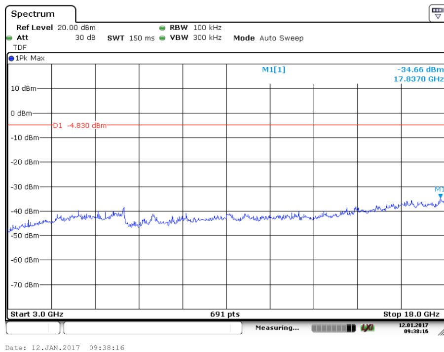
Fig. 27 Conducted Spurious Emission (GFSK, Ch39, 3GHz-18 GHz)
