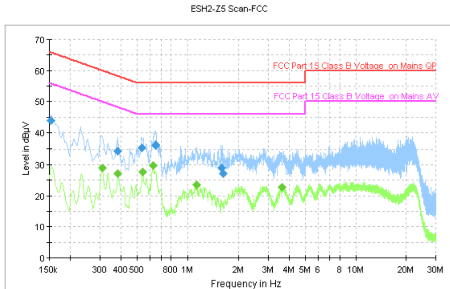
Fig. 102 AC Powerline Conducted Emission (Traffic, AE3)
