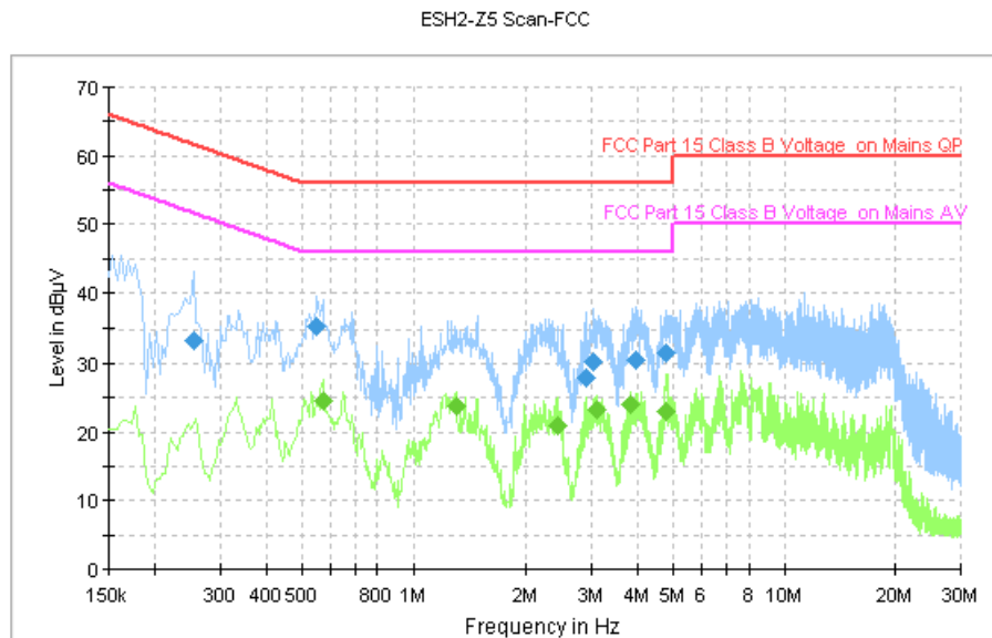
Fig. 100 AC Powerline Conducted Emission (Traffic, AE2)
