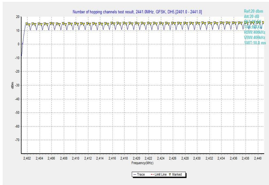
Fig. 89 Hopping channel ch0~39 (GFSK, Ch39)
