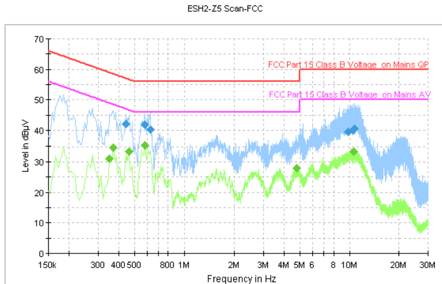
Fig. 98 AC Powerline Conducted Emission (Traffic, AE1)
