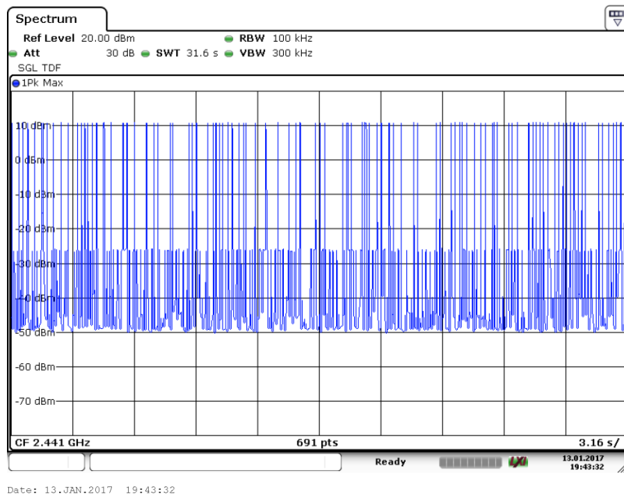
Fig. 86 Number of Transmissions ( \pi/4 DQPSK, Ch39)
