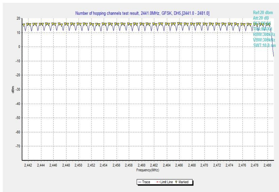
Fig. 90 Hopping channel ch39~78 (GFSK, Ch39)
