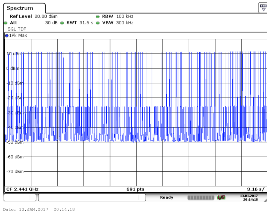
Fig. 88 Number of Transmissions (8DPSK, Ch39)
