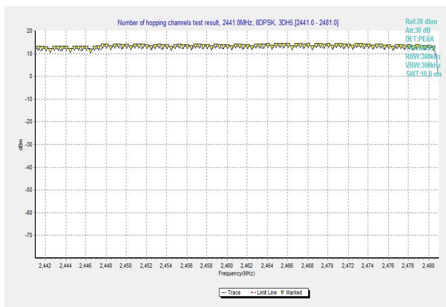
Fig. 94 Hopping channel ch39~78 (8DPSK, Ch39)
