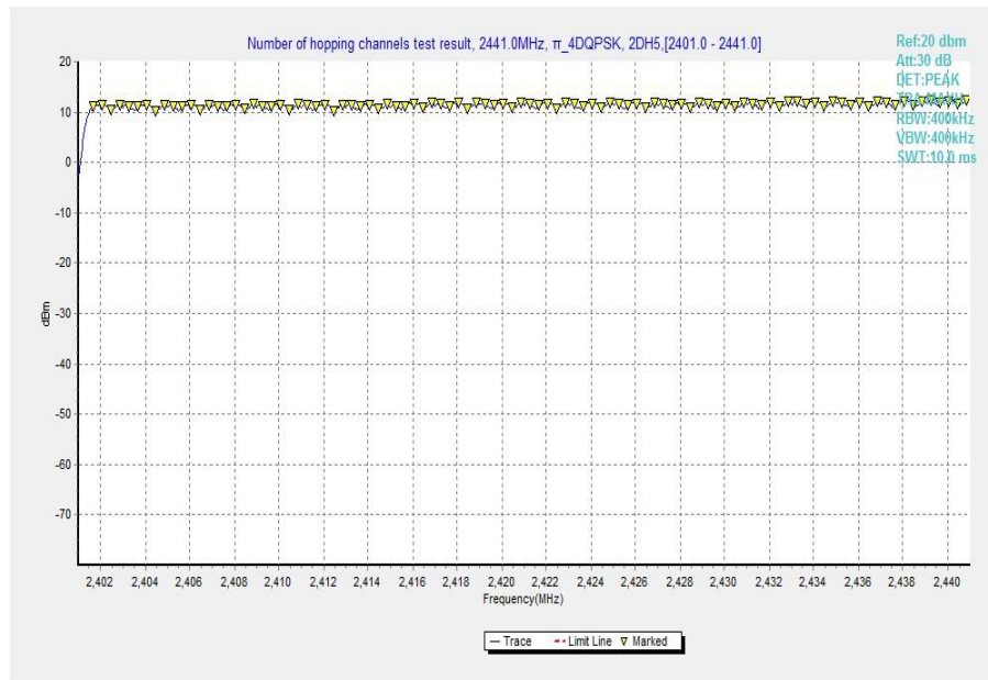
Fig. 91 Hopping channel ch0~39 ( \pi/4 DQPSK, Ch39)
