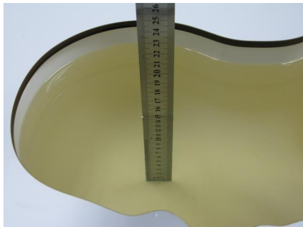
Photo 9: MSL 2450MHz Depth (15.1cm)
