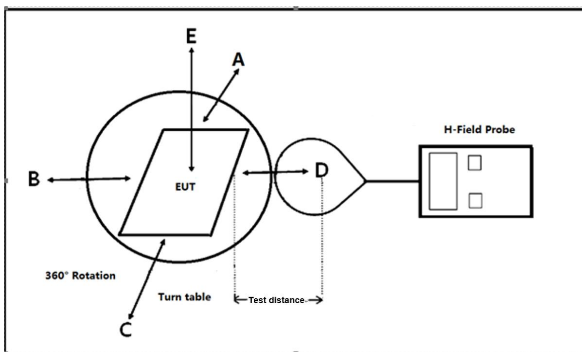
Figure: Test set-up
