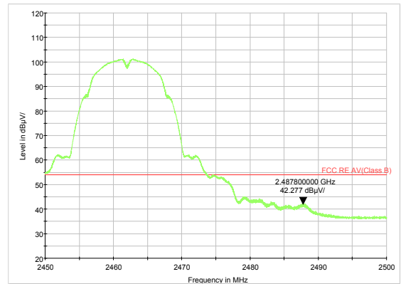
802.11b-Channel 11 Average
