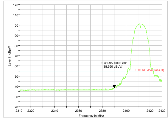
802.11b-Channel 1 Average
