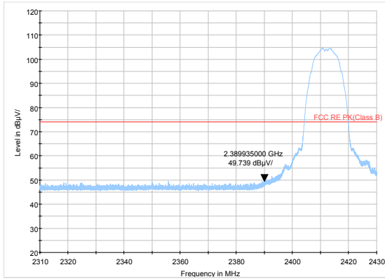
802.11b-Channel 1 Peak
