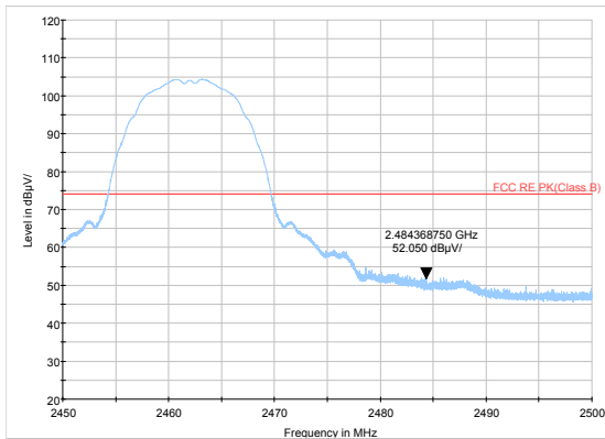
802.11b-Channel 11 Peak
