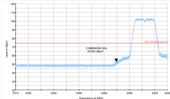
802.11g-Channel 1 Peak
