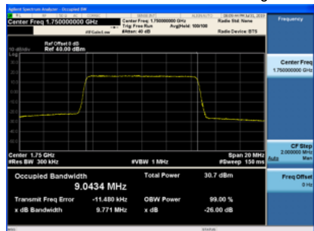
LTE Band 4 64QAM 10MHz CH-High
