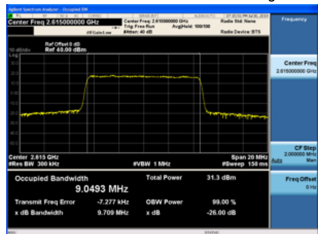
LTE Band 38 16QAM 10MHz CH-High
