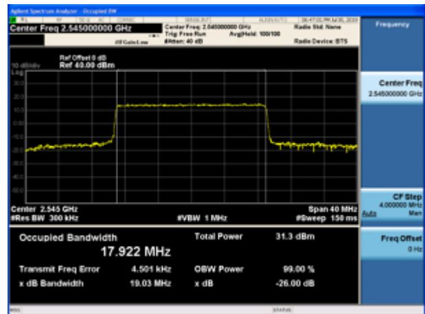
LTE Band 41 16QAM 20MHz CH-Middle
