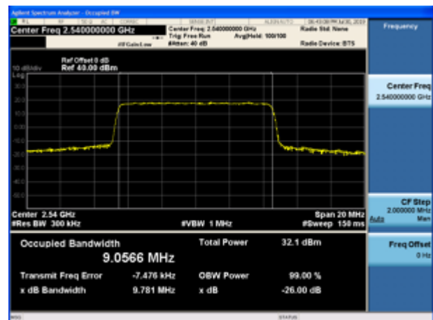
LTE Band 41 QPSK 10MHz CH-Middle
