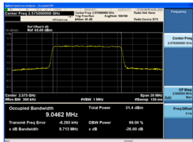
LTE Band 38 16QAM 10MHz CH-Middle
