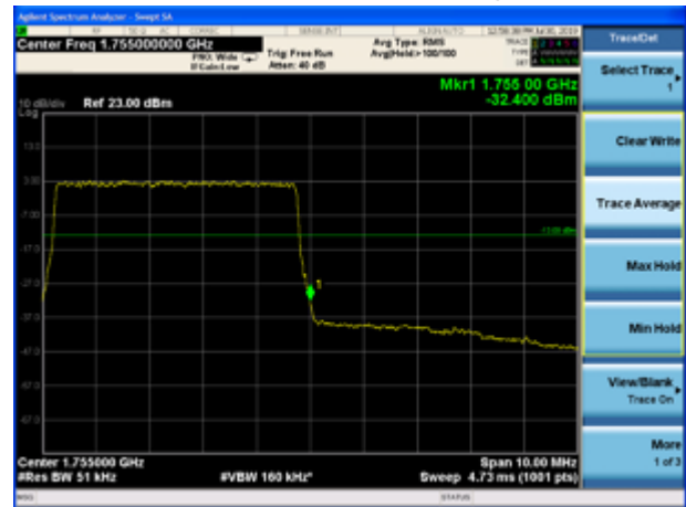
LTE Band 4 64QAM 10MHz CH-High, 1 RB
