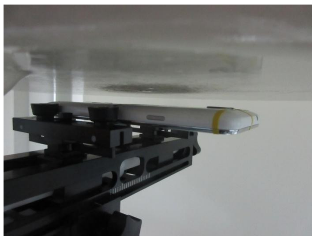
Photo 10: Right Side_10mm
