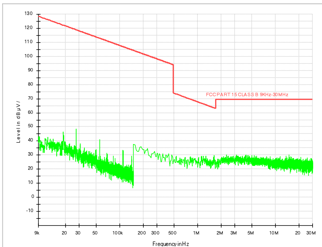
LTE FDD RSE-TX-DIRECTOR BELOW 1G_L
