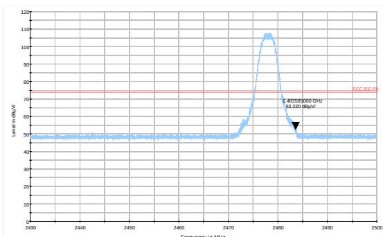
BT 2MHz 8DPSK(6Mbps) 2478MHz: Peak
