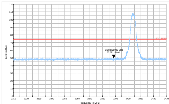
BT 2MHz \pi/4 -DQPSK(4Mbps) 2404MHz: Peak
