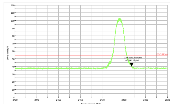
BT 2MHz 8DPSK(6Mbps) 2478MHz: Average
