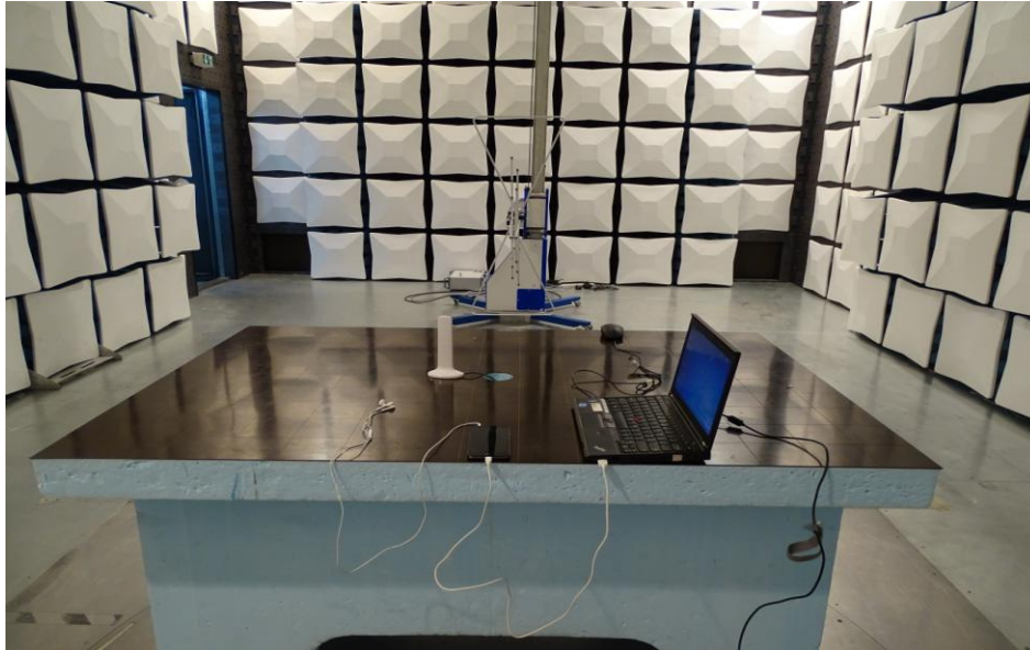
Radiated Spurious Emission (below 1GHz)
