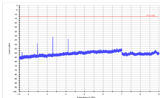
LTE Band 5 3MHz CH-Middle 1.5GHz~9GHz
