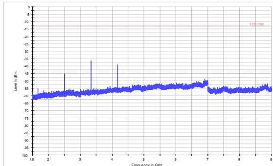
LTE Band 5 5MHz CH-High 1.5GHz~9GHz
