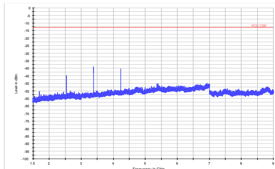
LTE Band 5 3MHz CH-High 1.5GHz~9GHz
