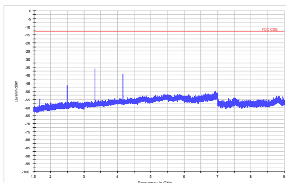
LTE Band 5 10MHz CH-High 1.5GHz~9GHz
