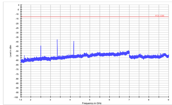
LTE Band 5 1.4MHz CH-High 1.5GHz~9GHz
