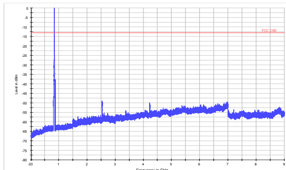
WCDMA Band V CH-High 30MHz~9GHz
