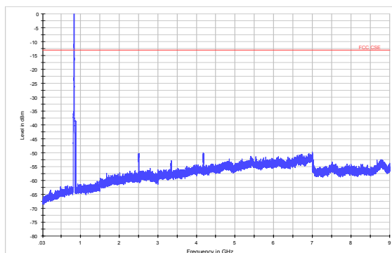
WCDMA Band V CH-High 30MHz~9GHz
