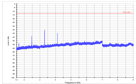
LTE Band 5 1.4MHz CH-Middle 1.5GHz~9GHz
