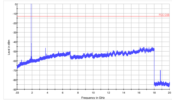
GSM 1900 CH-High 30MHz~20GHz
