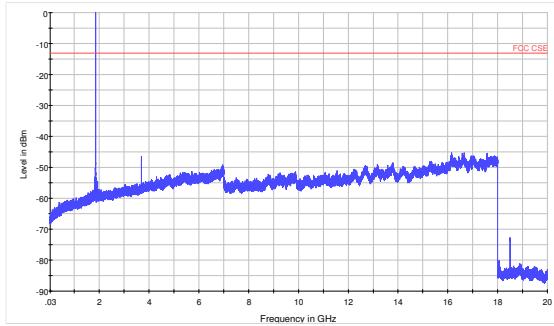
GSM 1900 CH-High 30MHz~20GHz
