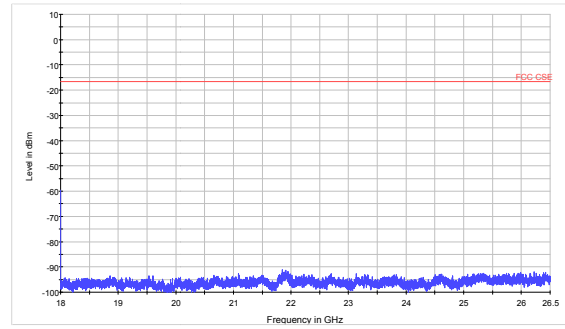
EDR-CH39 18GHz to 26.5GHz
