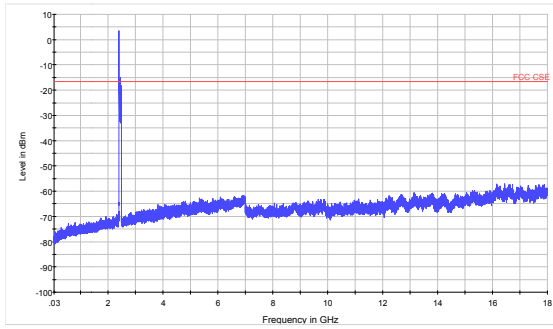
EDR-CH39 30MHz to 18GHz
