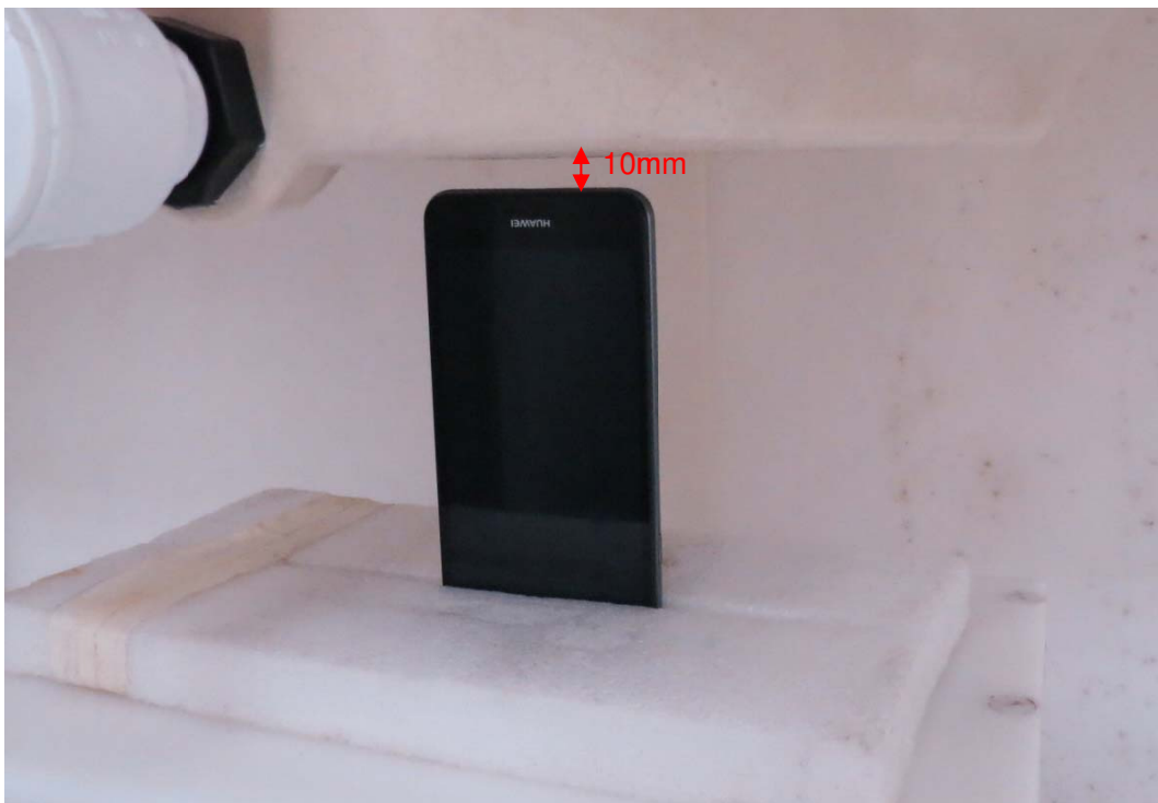
Picture 13: Bottom Side, the distance from handset to the bottom of the Phantom is 10mm
