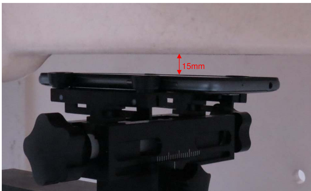
Picture 7: Front Side, the distance from handset to the bottom of the Phantom is 15mm
