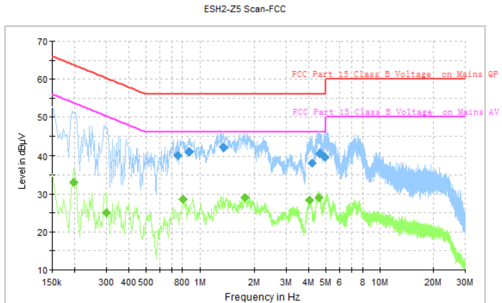
Figure A.17 Conducted Emission
