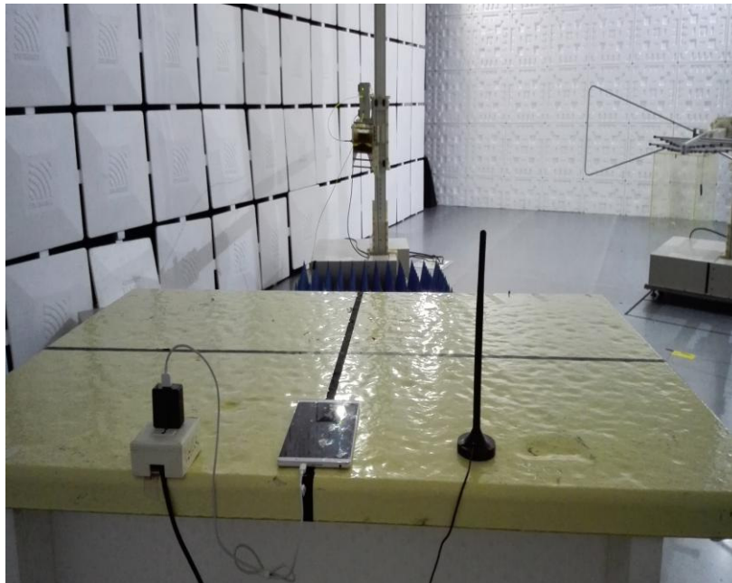
Radiated Spurious Emission (1GHz to 18GHz)
