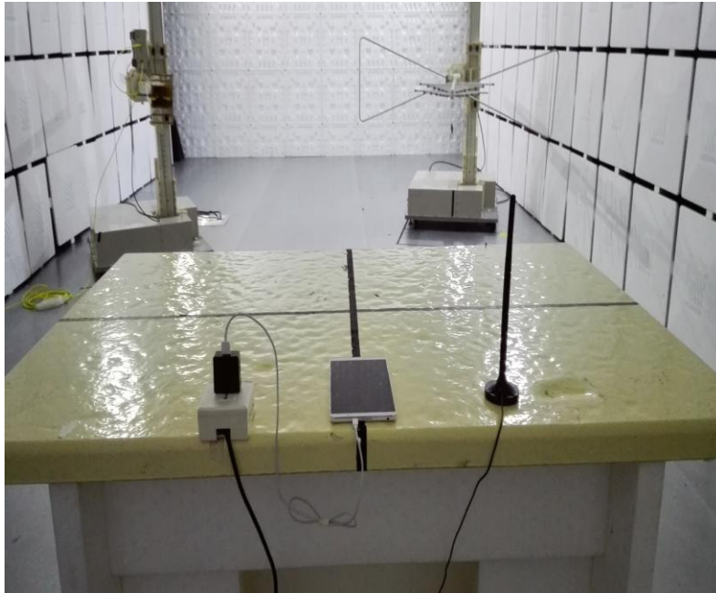
Radiated Spurious Emission (below 1GHz)
