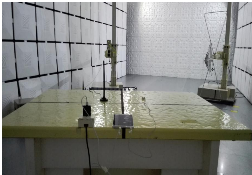
Radiated Spurious Emission (above 18GHz)
