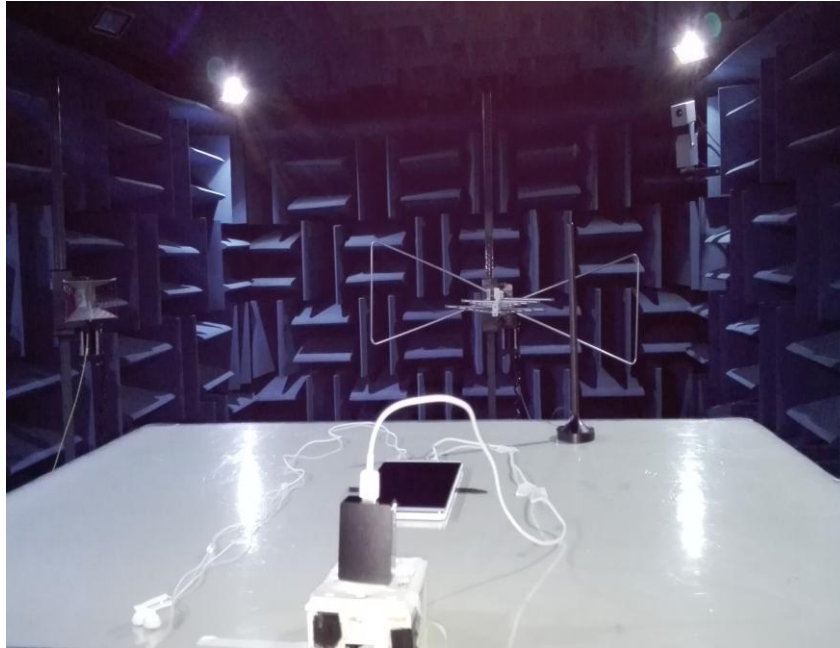
Radiated Spurious Emission (below 1GHz)
