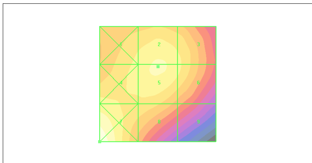
Figure 36 HAC RF H-Field CDMA PCS Channel 1175
