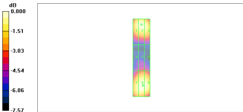
Figure 12 System Performance Check 1880MHz_E
