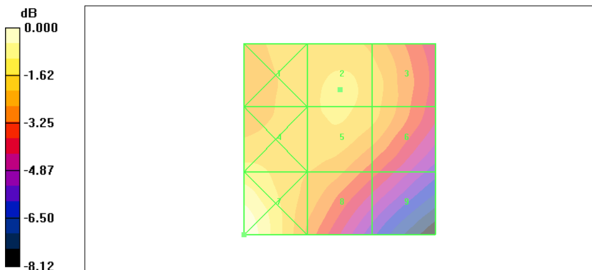
Figure 33 HAC RF H-Field CDMA PCS Channel 600
