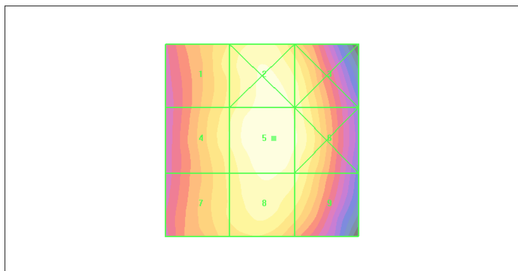
Figure 17 HAC RF E-Field CDMA Cellular Channel 384
