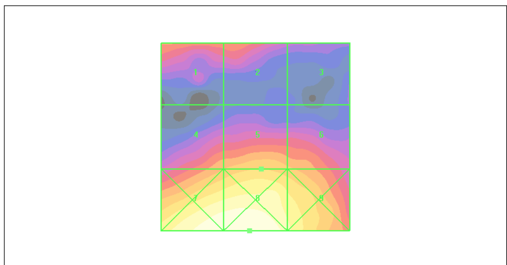
Figure 41 HAC RF E-Field CDMA AWS Channel 25
