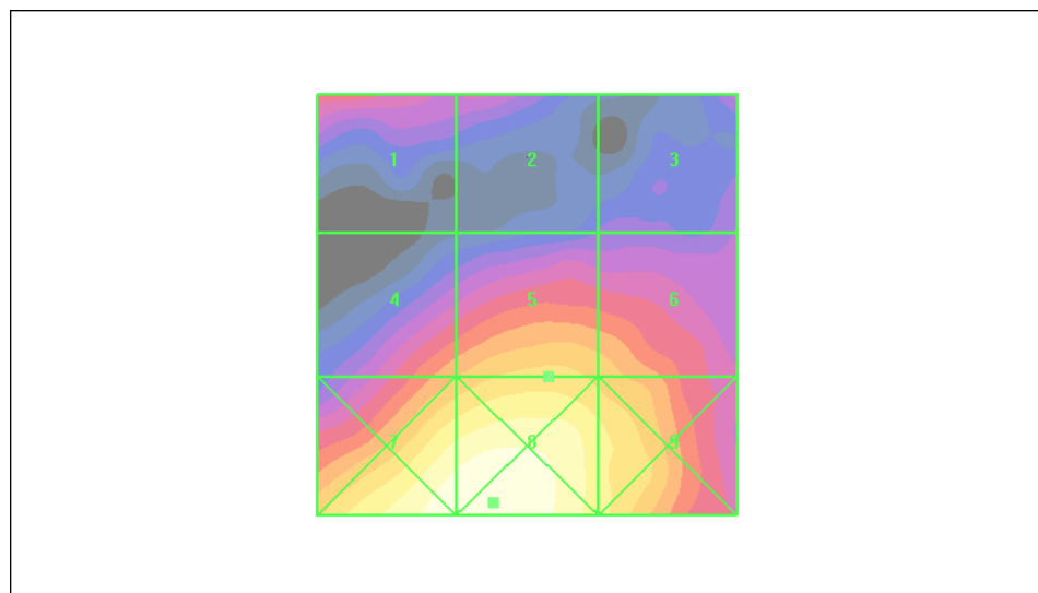
Figure 27 HAC RF E-Field CDMA PCS Channel 600
