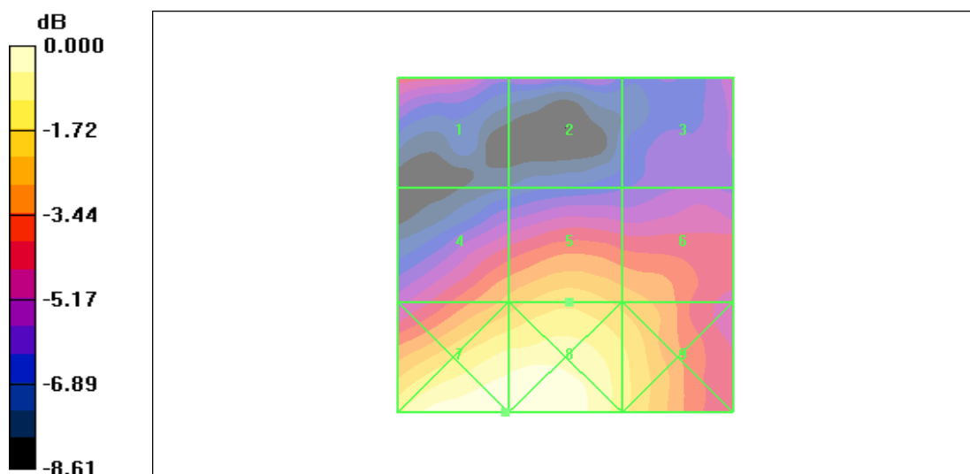
Figure 28 HAC RF E-Field CDMA PCS Channel 25
