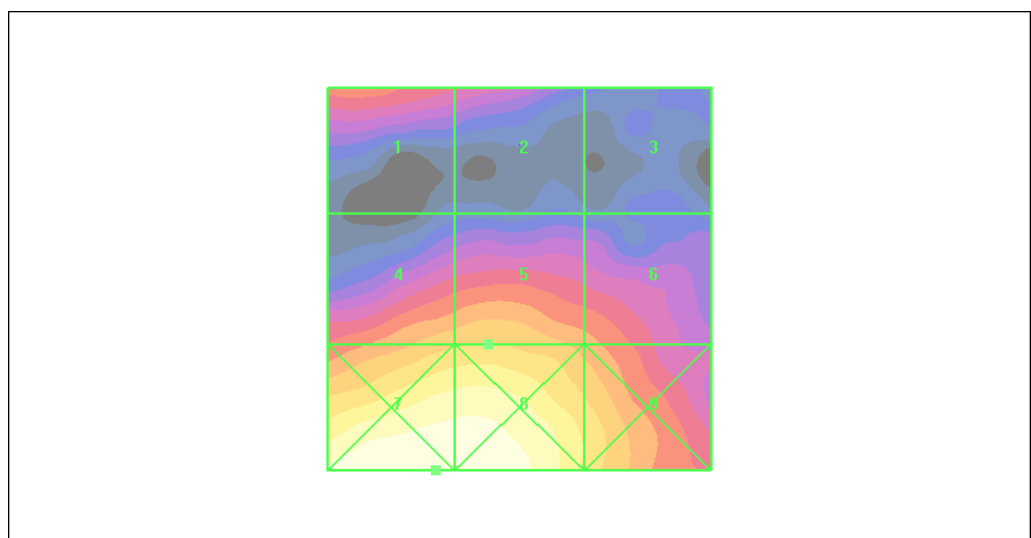
Figure 42 HAC RF E-Field CDMA AWS Channel 25
