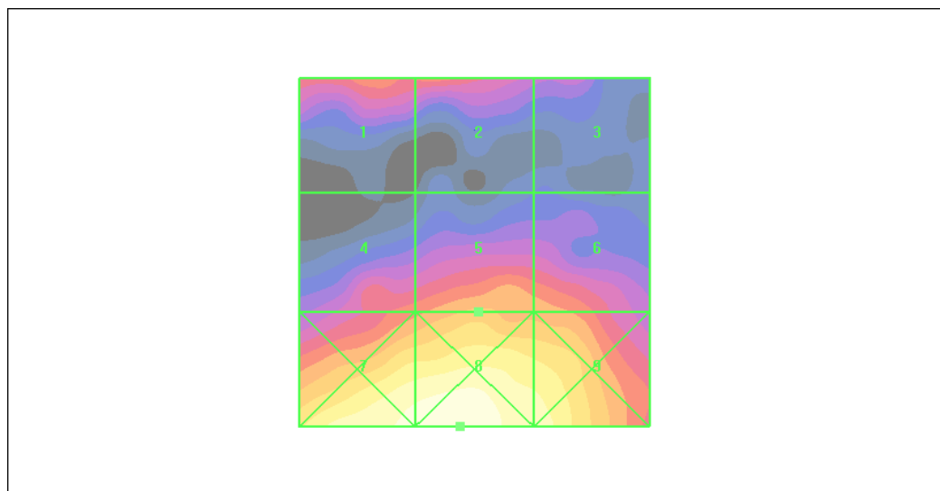
Figure 39 HAC RF E-Field CDMA AWS Channel 450
