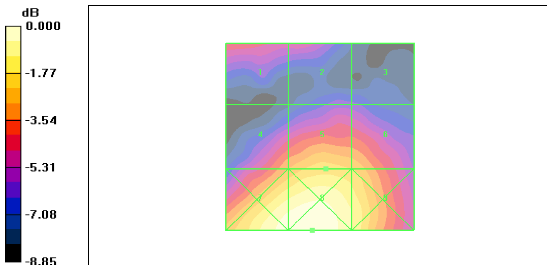
Figure 26 HAC RF E-Field CDMA PCS Channel 1175
