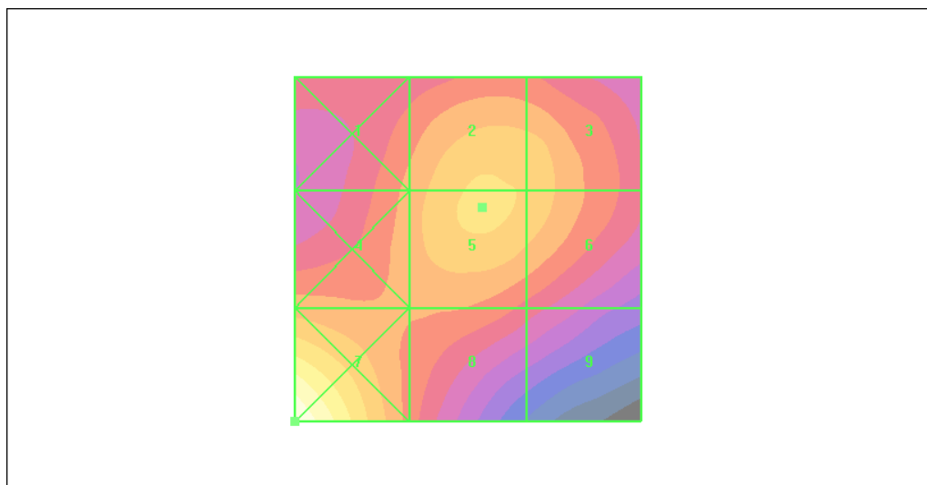
Figure 45 HAC RF H-Field CDMA AWS Channel 450
