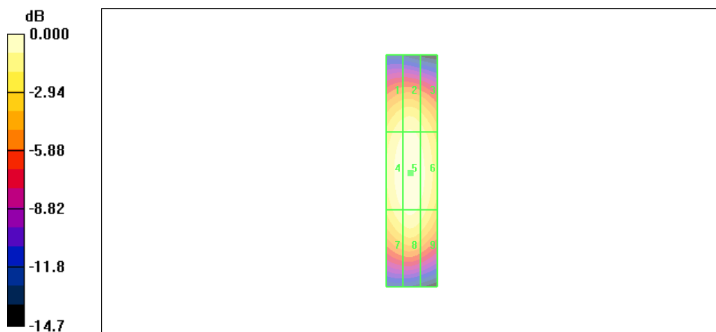
Figure 13 System Performance Check 1880MHz_H
