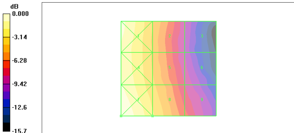
Figure 20 HAC RF H-Field CDMA Cellular Channel 777
