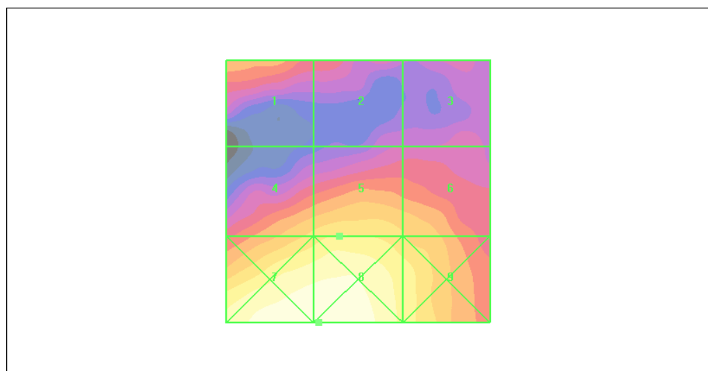
Figure 31 HAC RF E-Field CDMA PCS Channel 1175
