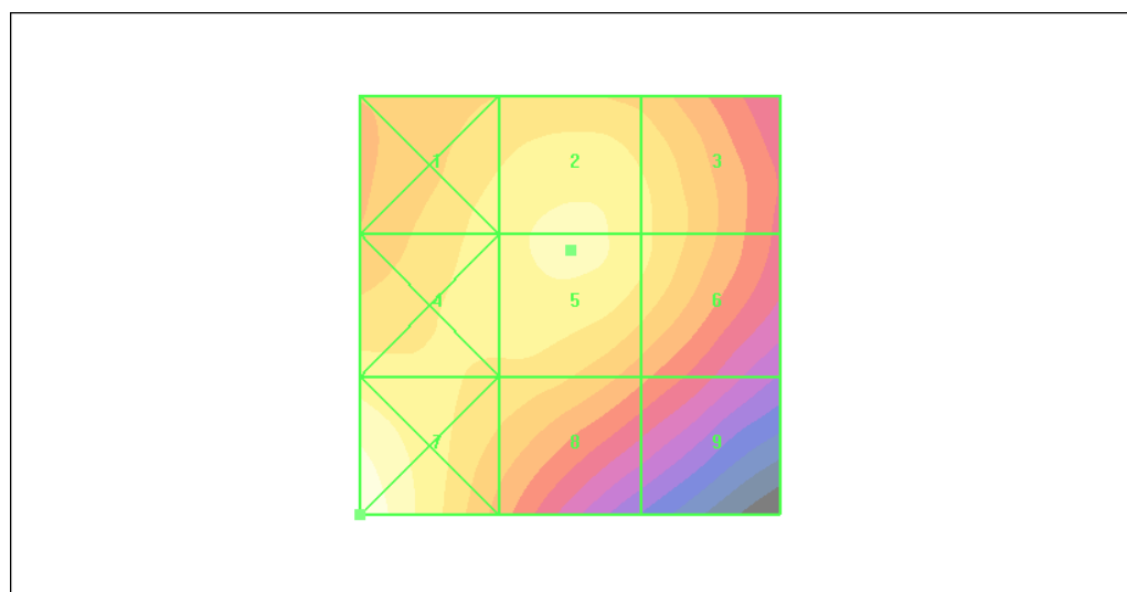
Figure 32 HAC RF H-Field CDMA PCS Channel 1175
