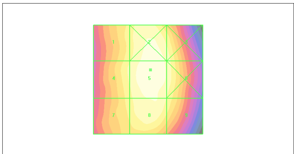
Figure 19 HAC RF E-Field CDMA Cellular Channel 384
