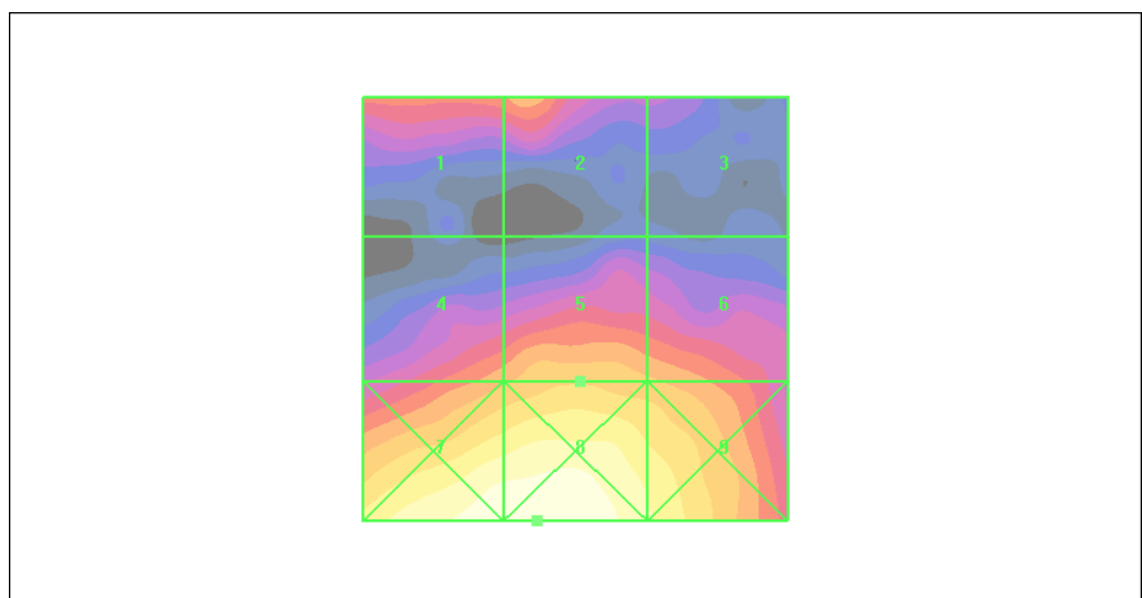
Figure 40 HAC RF E-Field CDMA AWS Channel 25
