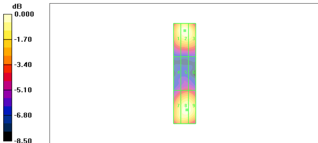
Figure 11 System Performance Check 1880MHz_E
