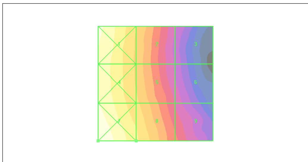
Figure 21 HAC RF H-Field CDMA Cellular Channel 384
