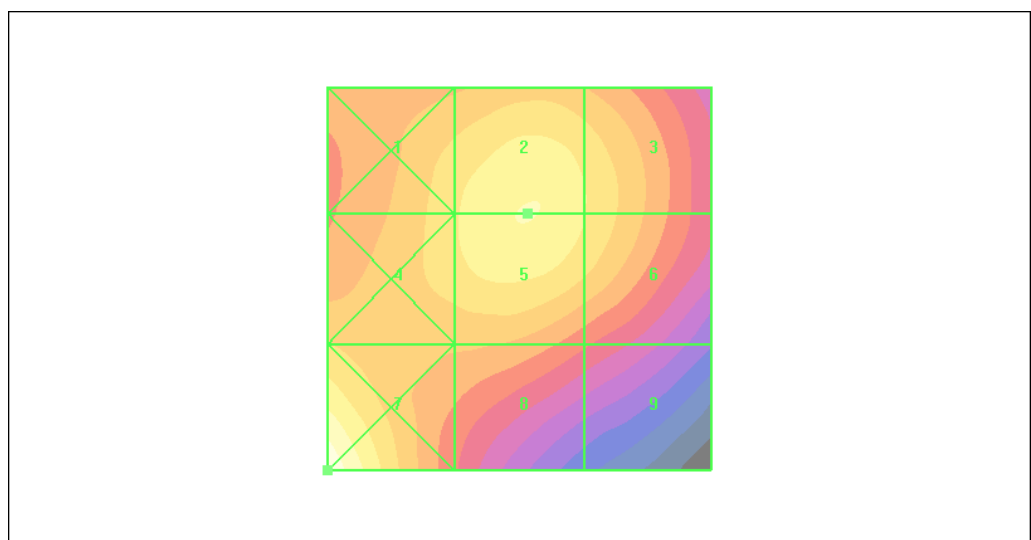
Figure 47 HAC RF H-Field CDMA AWS Channel 25
