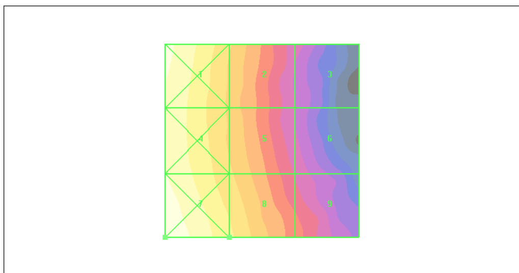
Figure 22 HAC RF H-Field CDMA Cellular Channel 1013
