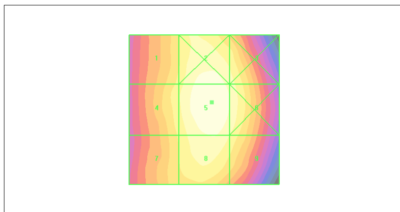
Figure 14 HAC RF E-Field CDMA Cellular Channel 777
