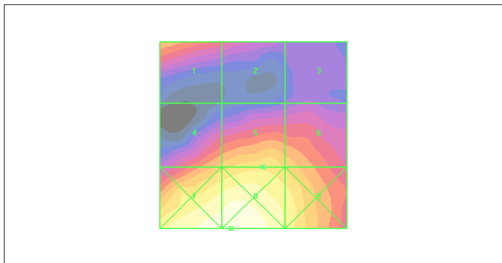
Figure 29 HAC RF E-Field CDMA PCS Channel 1175
