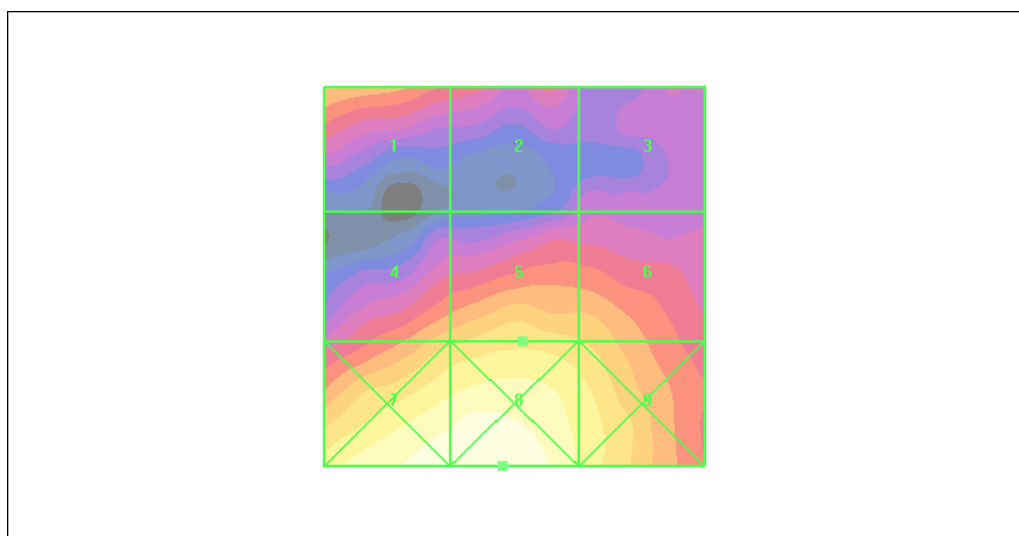
Figure 30 HAC RF E-Field CDMA PCS Channel 1175
