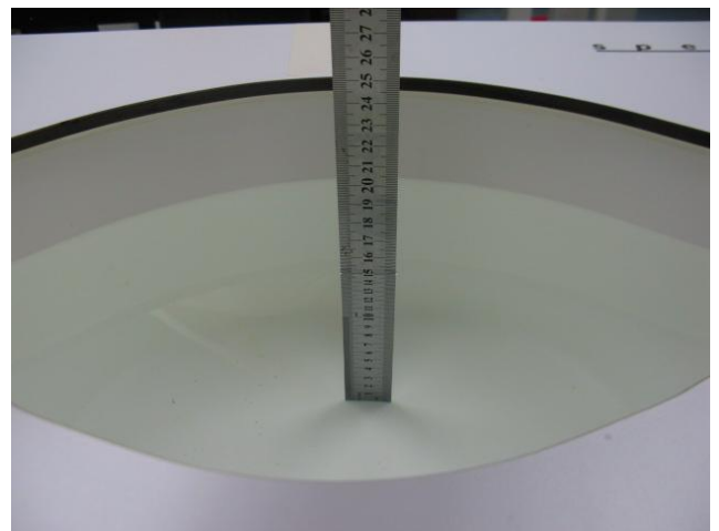
Photo 15: MSL1800MHz depth (15.2cm)
