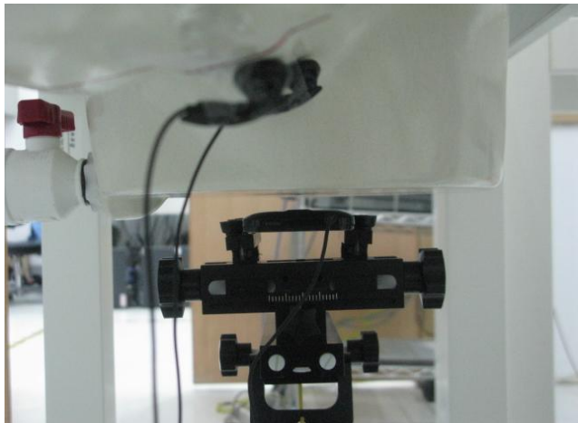
Photo 13: Towards Ground with Headset (10mm)
