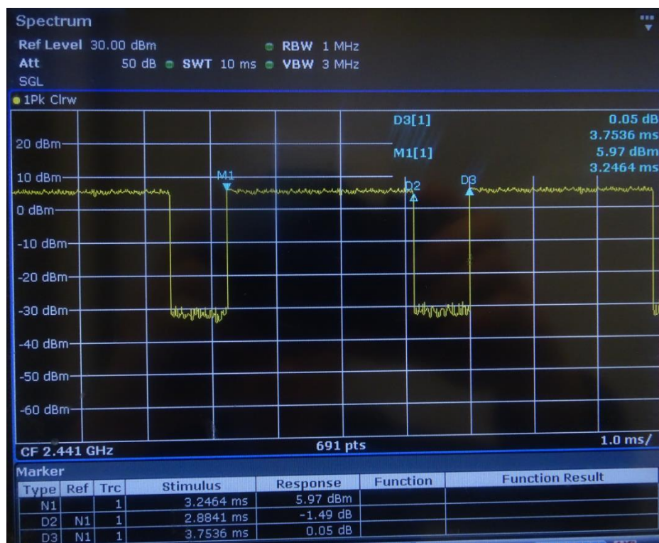
Figure: Bluetooth Transmission Plot
