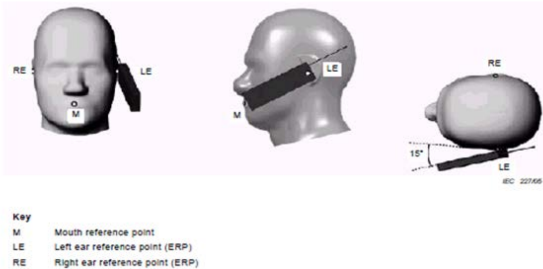
Figure 1-2 Tilt position of the wireless device on the left side of SAM
