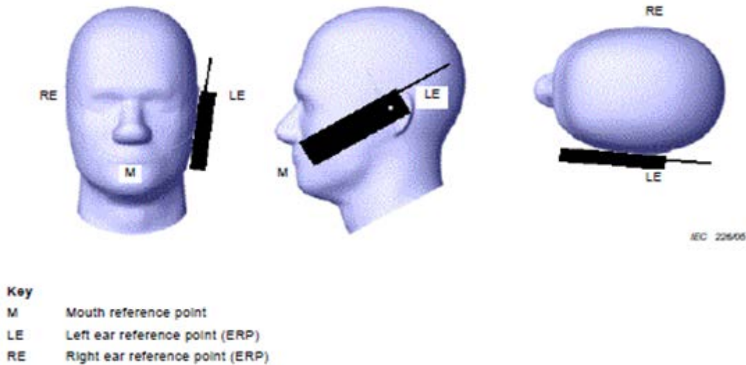
Figure 1-1 Cheek position of the wireless device on the left side of SAM
