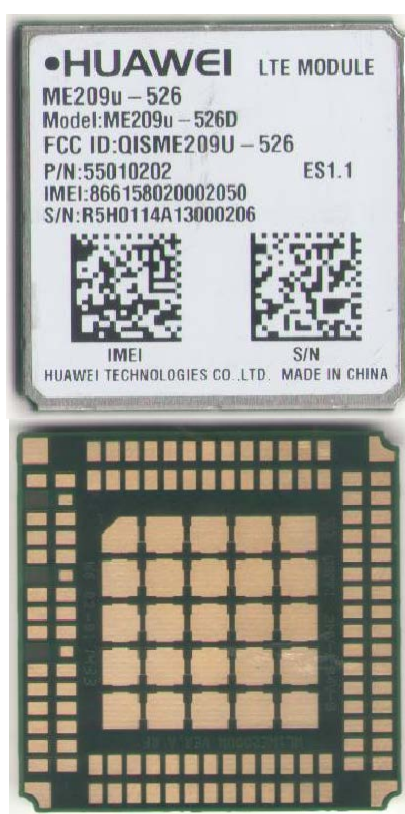
Figure1 EUT Appearance
