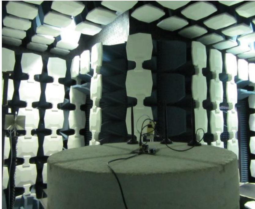
Radiated Spurious Emission (18GHz to 26.5GHz)
