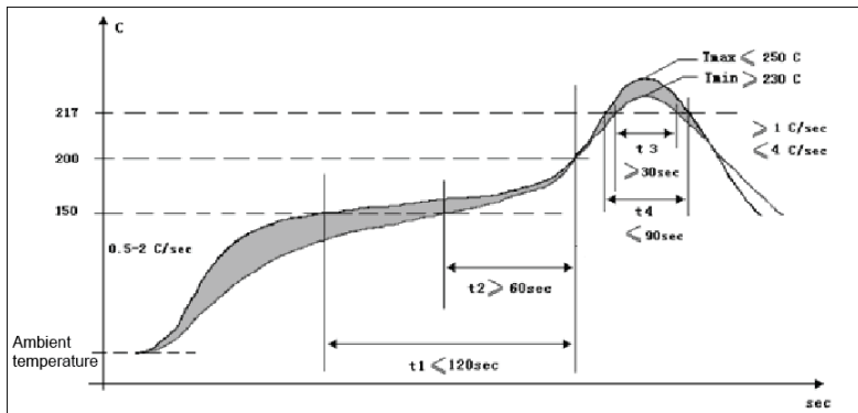
Reflow profile
